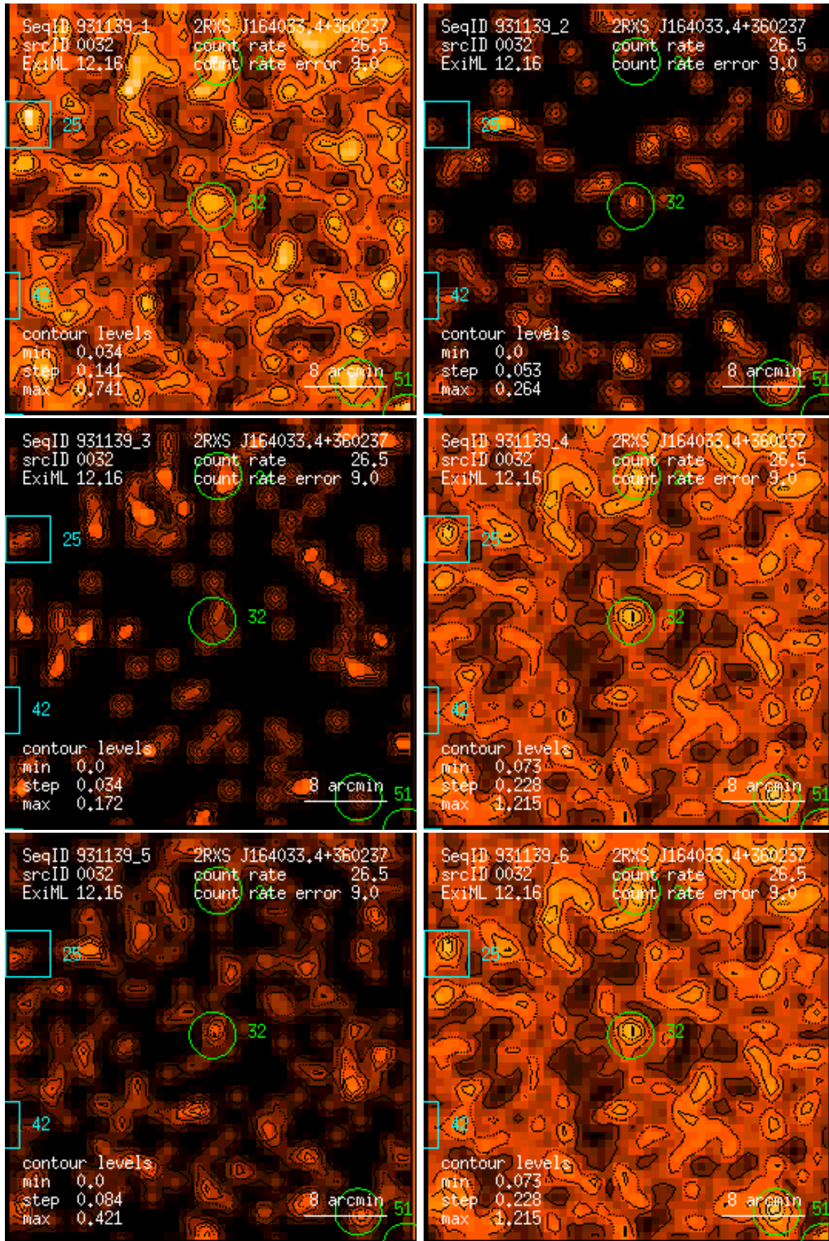
Figure 32: RASS 931139: detection 0032: band rate images, Gaussian filter: (1) PSPC channels 11 – 41, (2) 52 – 90, (3) 91 – 201, (4) 11 – 235, (5) 52 – 201, (6) 11 – 201. Broad band rates in counts/ks. Band rate contour levels in counts/ks/arcmin 2 .
