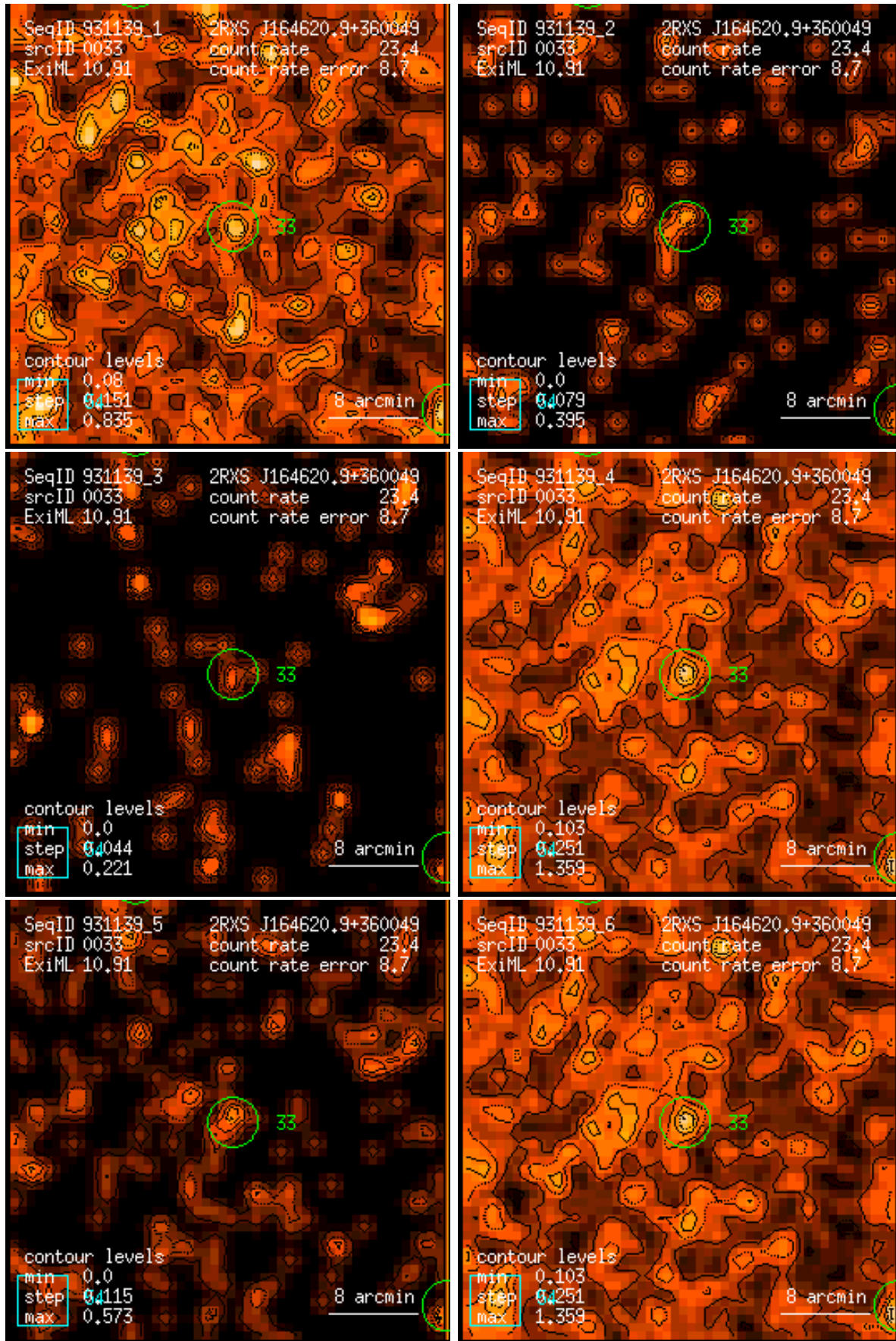
Figure 33: RASS 931139: detection 0033: band rate images, Gaussian filter: (1) PSPC channels 11 – 41, (2) 52 – 90, (3) 91 – 201, (4) 11 – 235, (5) 52 – 201, (6) 11 – 201. Broad band rates in counts/ks. Band rate contour levels in counts/ks/arcmin 2 .
