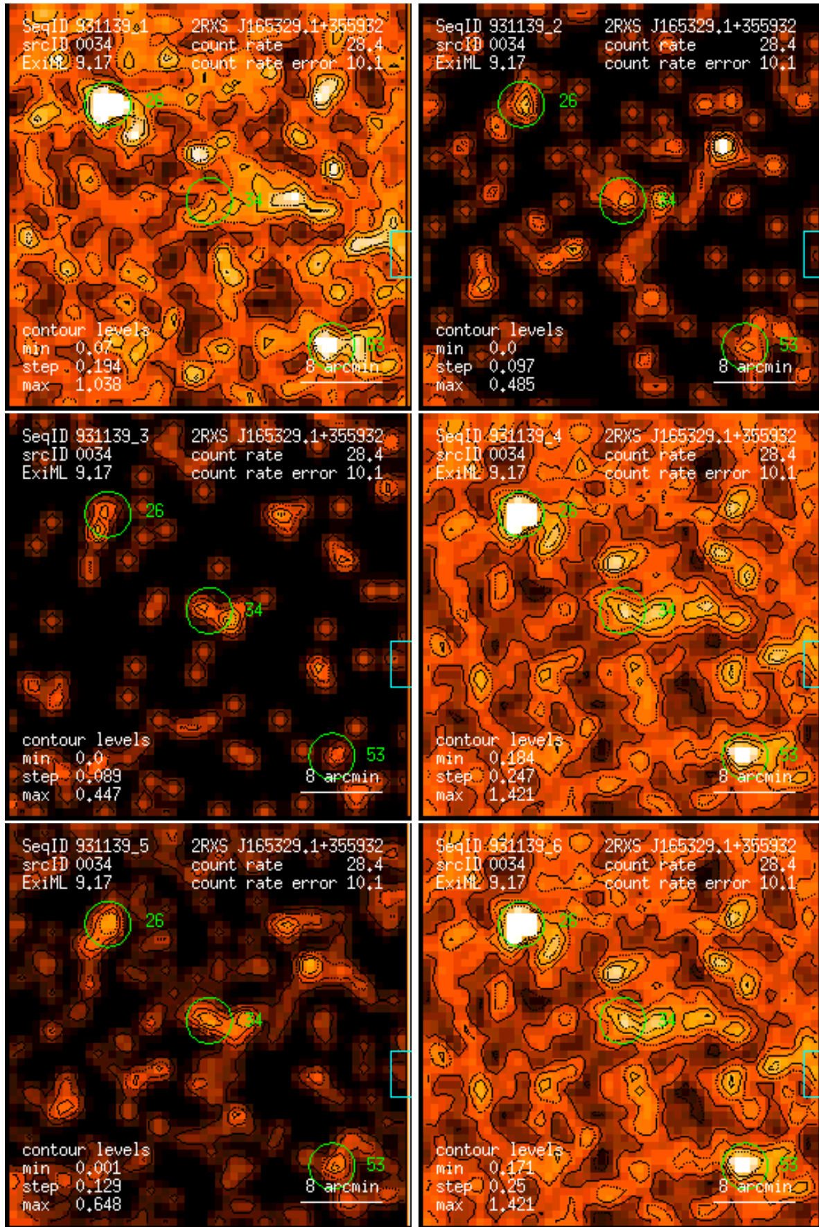
Figure 34: RASS 931139: detection 0034: band rate images, Gaussian filter: (1) PSPC channels 11 – 41, (2) 52 – 90, (3) 91 – 201, (4) 11 – 235, (5) 52 – 201, (6) 11 – 201. Broad band rates in counts/ks. Band rate contour levels in counts/ks/arcmin 2 .
