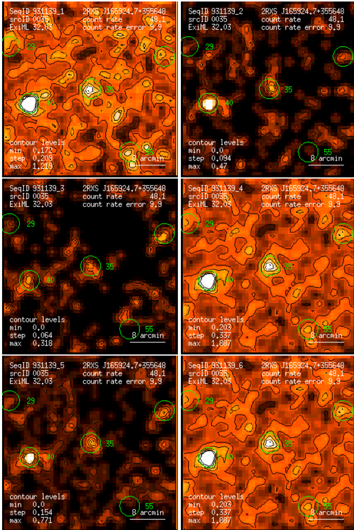
Figure 35: RASS 931139: detection 0035: band rate images, Gaussian filter: (1) PSPC channels 11 – 41, (2) 52 – 90, (3) 91 – 201, (4) 11 – 235, (5) 52 – 201, (6) 11 – 201. Broad band rates in counts/ks. Band rate contour levels in counts/ks/arcmin 2 .
