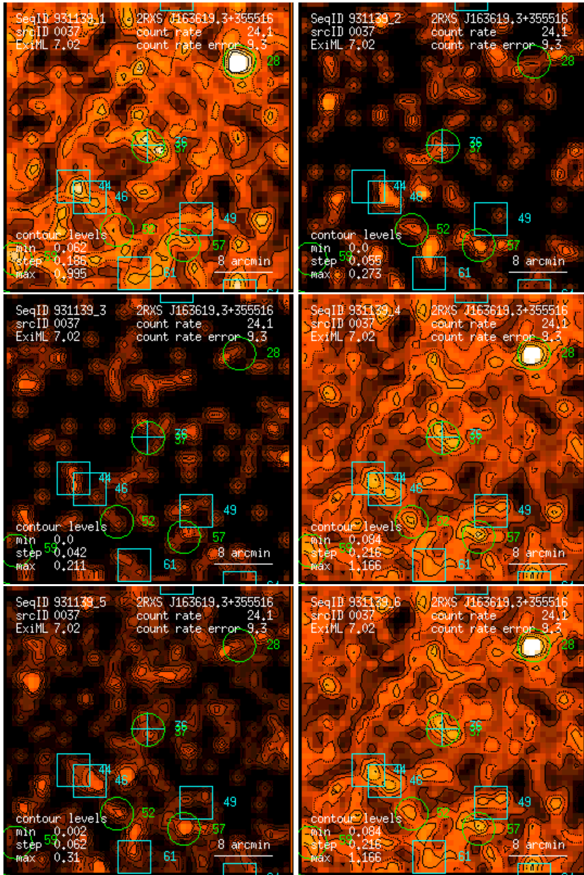
Figure 37: RASS 931139: detection 0037: band rate images, Gaussian filter: (1) PSPC channels 11 – 41, (2) 52 – 90, (3) 91 – 201, (4) 11 – 235, (5) 52 – 201, (6) 11 – 201. Broad band rates in counts/ks. Band rate contour levels in counts/ks/arcmin 2 .
