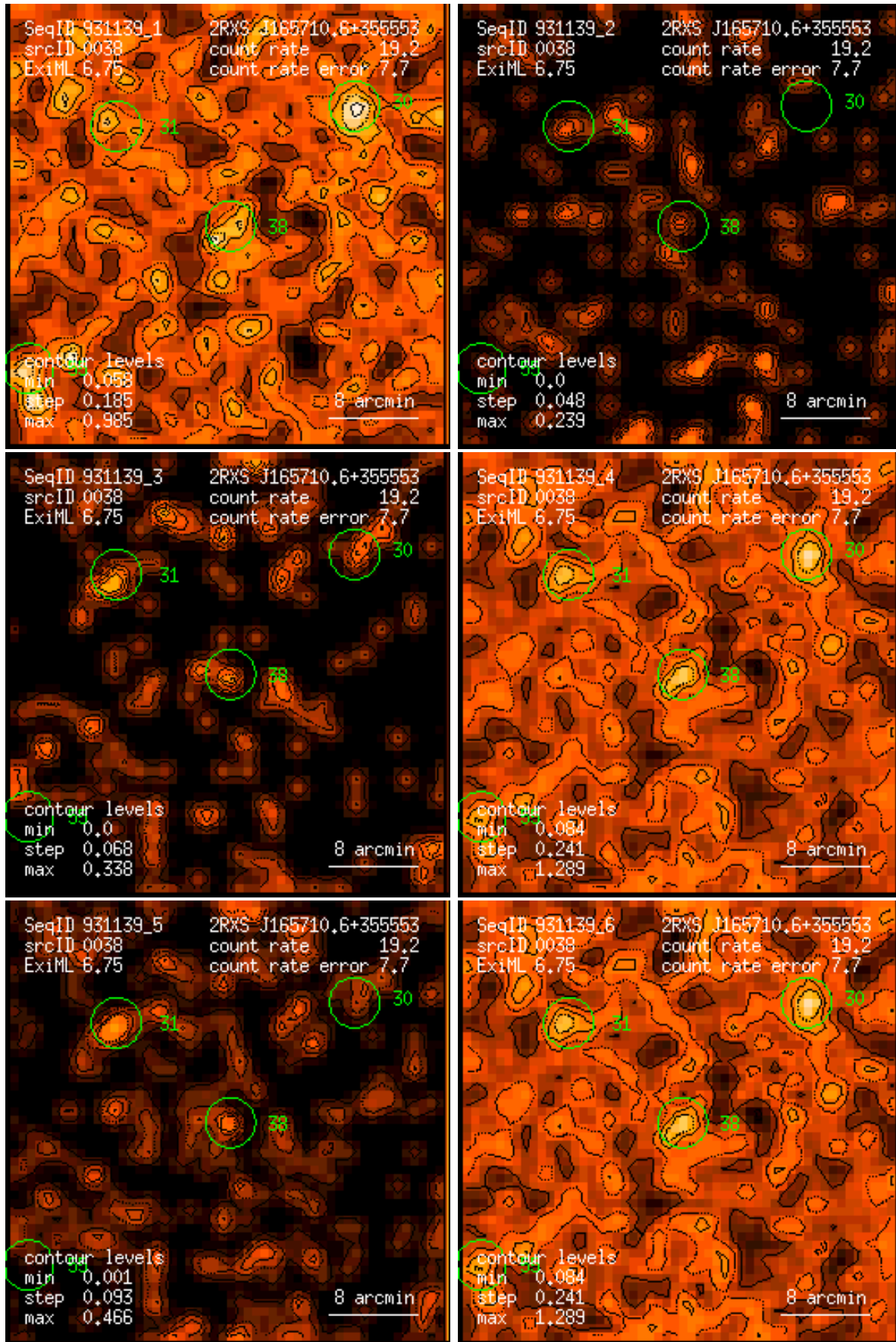
Figure 38: RASS 931139: detection 0038: band rate images, Gaussian filter: (1) PSPC channels 11 – 41, (2) 52 – 90, (3) 91 – 201, (4) 11 – 235, (5) 52 – 201, (6) 11 – 201. Broad band rates in counts/ks. Band rate contour levels in counts/ks/arcmin 2 .
