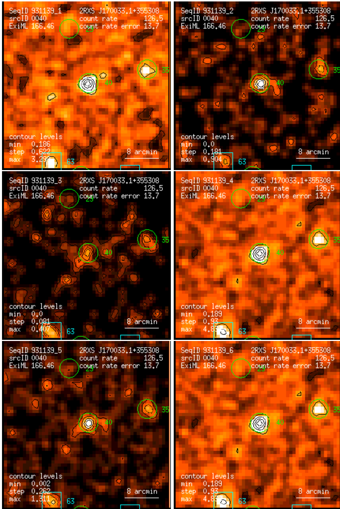
Figure 40: RASS 931139: detection 0040: band rate images, Gaussian filter: (1) PSPC channels 11 – 41, (2) 52 – 90, (3) 91 – 201, (4) 11 – 235, (5) 52 – 201, (6) 11 – 201. Broad band rates in counts/ks. Band rate contour levels in counts/ks/arcmin 2 .
