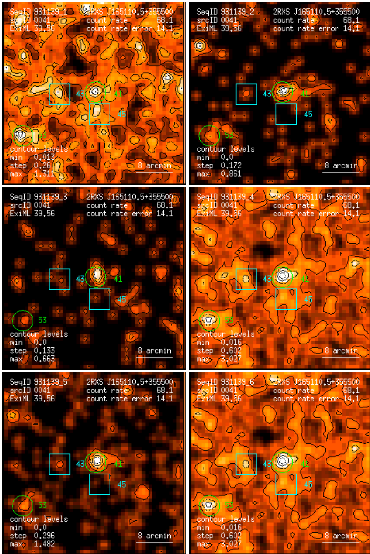
Figure 41: RASS 931139: detection 0041: band rate images, Gaussian filter: (1) PSPC channels 11 – 41, (2) 52 – 90, (3) 91 – 201, (4) 11 – 235, (5) 52 – 201, (6) 11 – 201. Broad band rates in counts/ks. Band rate contour levels in counts/ks/arcmin 2 .
