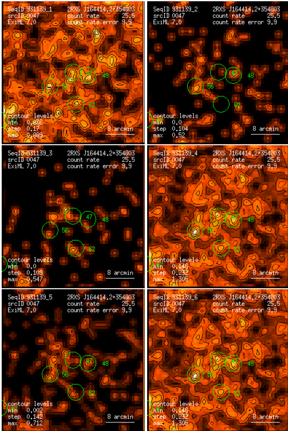
Figure 47: RASS 931139: detection 0047: band rate images, Gaussian filter: (1) PSPC channels 11 – 41, (2) 52 – 90, (3) 91 – 201, (4) 11 – 235, (5) 52 – 201, (6) 11 – 201. Broad band rates in counts/ks. Band rate contour levels in counts/ks/arcmin 2 .
