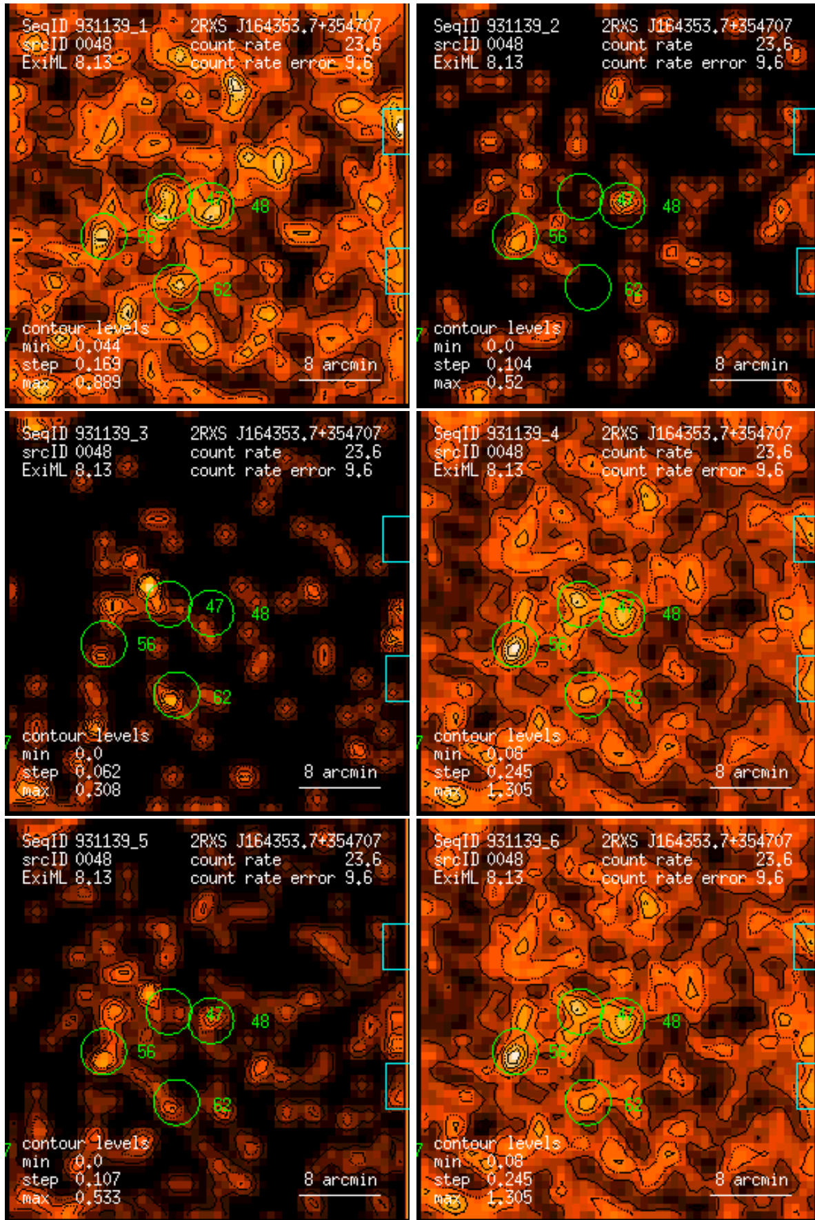
Figure 48: RASS 931139: detection 0048: band rate images, Gaussian filter: (1) PSPC channels 11 – 41, (2) 52 – 90, (3) 91 – 201, (4) 11 – 235, (5) 52 – 201, (6) 11 – 201. Broad band rates in counts/ks. Band rate contour levels in counts/ks/arcmin 2 .
