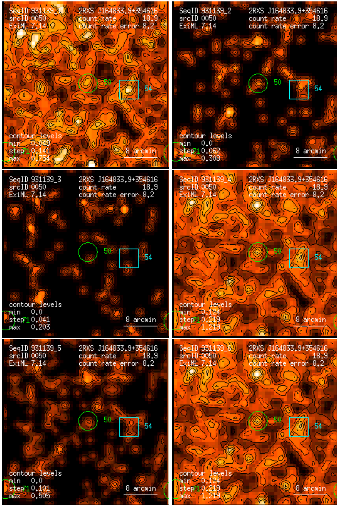
Figure 50: RASS 931139: detection 0050: band rate images, Gaussian filter: (1) PSPC channels 11 – 41, (2) 52 – 90, (3) 91 – 201, (4) 11 – 235, (5) 52 – 201, (6) 11 – 201. Broad band rates in counts/ks. Band rate contour levels in counts/ks/arcmin 2 .
