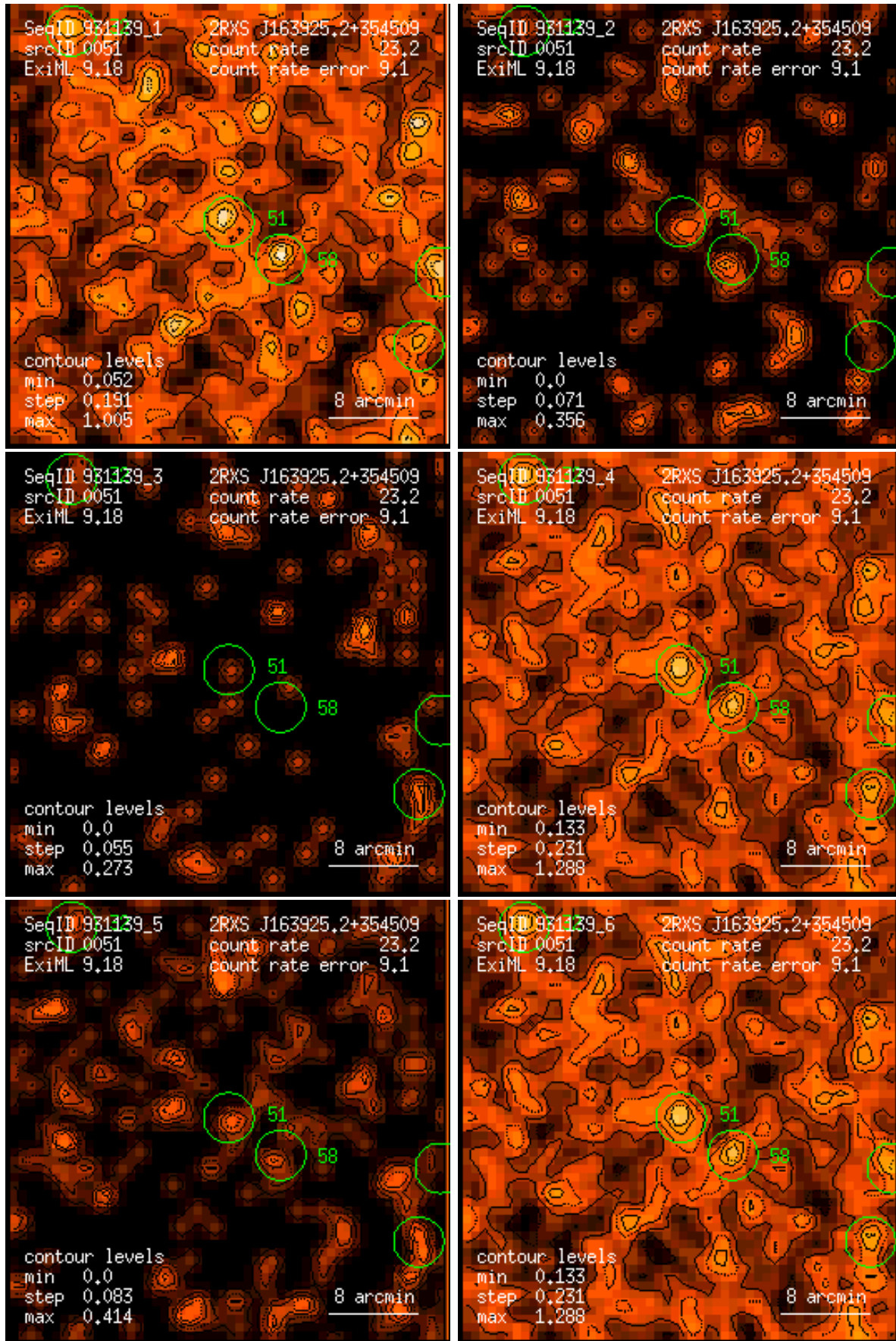
Figure 51: RASS 931139: detection 0051: band rate images, Gaussian filter: (1) PSPC channels 11 – 41, (2) 52 – 90, (3) 91 – 201, (4) 11 – 235, (5) 52 – 201, (6) 11 – 201. Broad band rates in counts/ks. Band rate contour levels in counts/ks/arcmin 2 .
