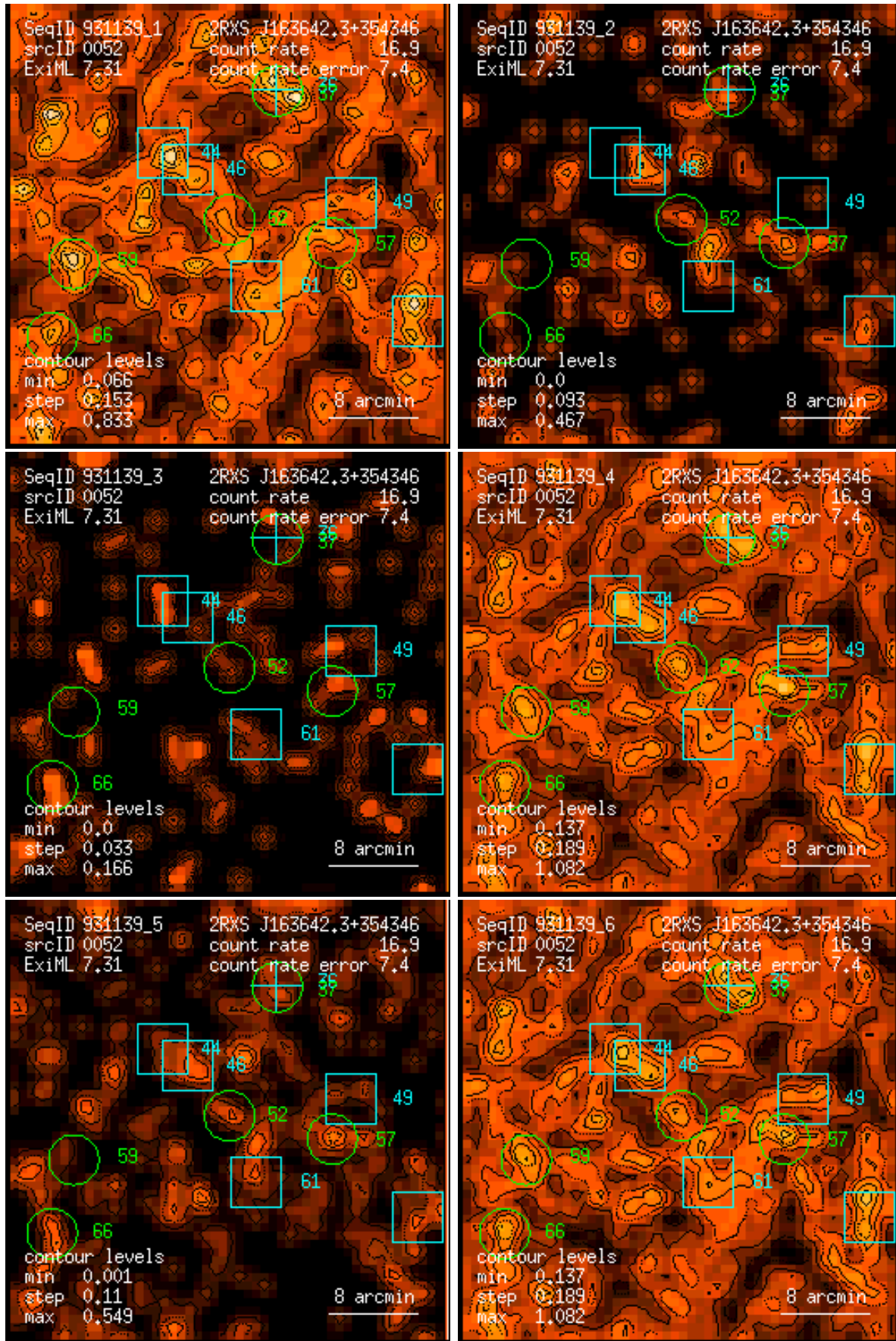
Figure 52: RASS 931139: detection 0052: band rate images, Gaussian filter: (1) PSPC channels 11 – 41, (2) 52 – 90, (3) 91 – 201, (4) 11 – 235, (5) 52 – 201, (6) 11 – 201. Broad band rates in counts/ks. Band rate contour levels in counts/ks/arcmin 2 .
