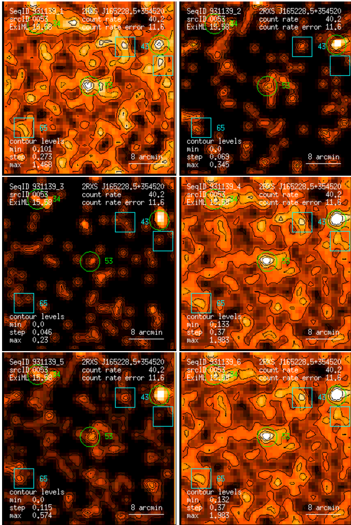
Figure 53: RASS 931139: detection 0053: band rate images, Gaussian filter: (1) PSPC channels 11 – 41, (2) 52 – 90, (3) 91 – 201, (4) 11 – 235, (5) 52 – 201, (6) 11 – 201. Broad band rates in counts/ks. Band rate contour levels in counts/ks/arcmin 2 .
