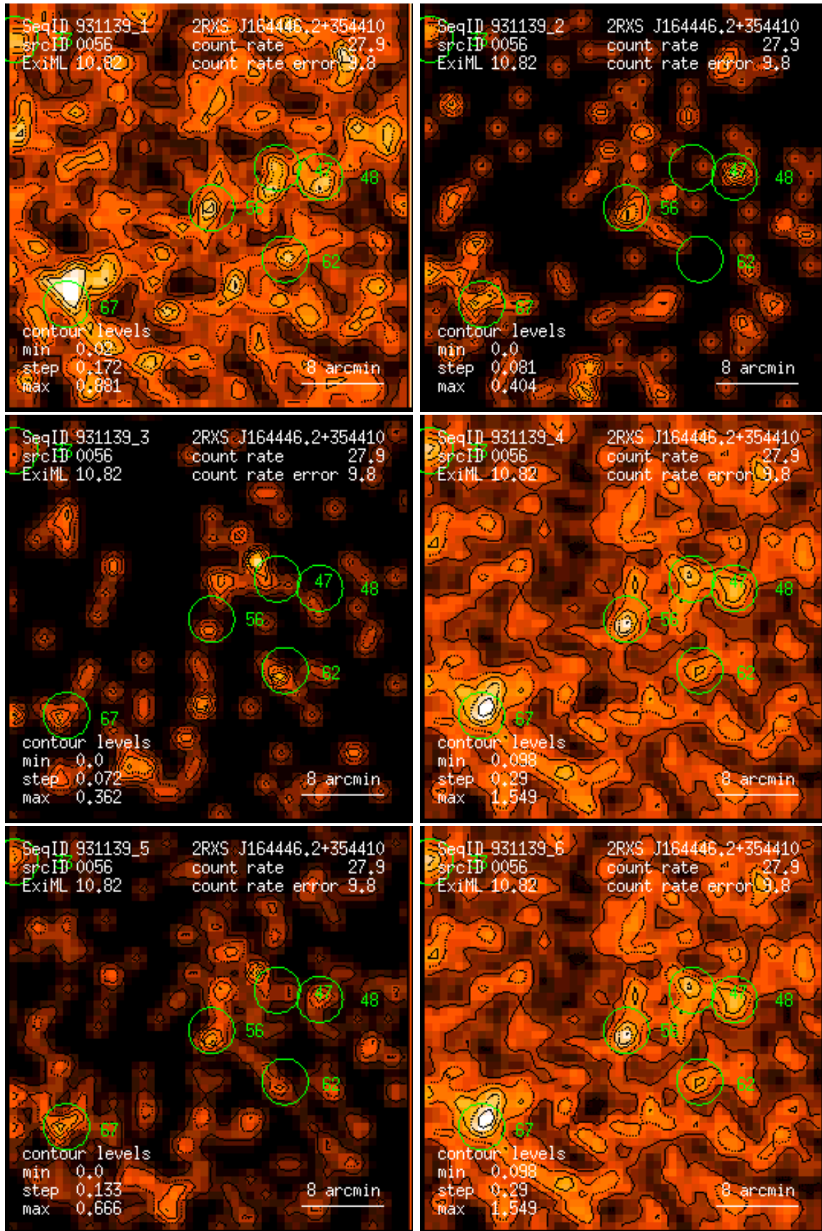
Figure 56: RASS 931139: detection 0056: band rate images, Gaussian filter: (1) PSPC channels 11 – 41, (2) 52 – 90, (3) 91 – 201, (4) 11 – 235, (5) 52 – 201, (6) 11 – 201. Broad band rates in counts/ks. Band rate contour levels in counts/ks/arcmin 2 .
