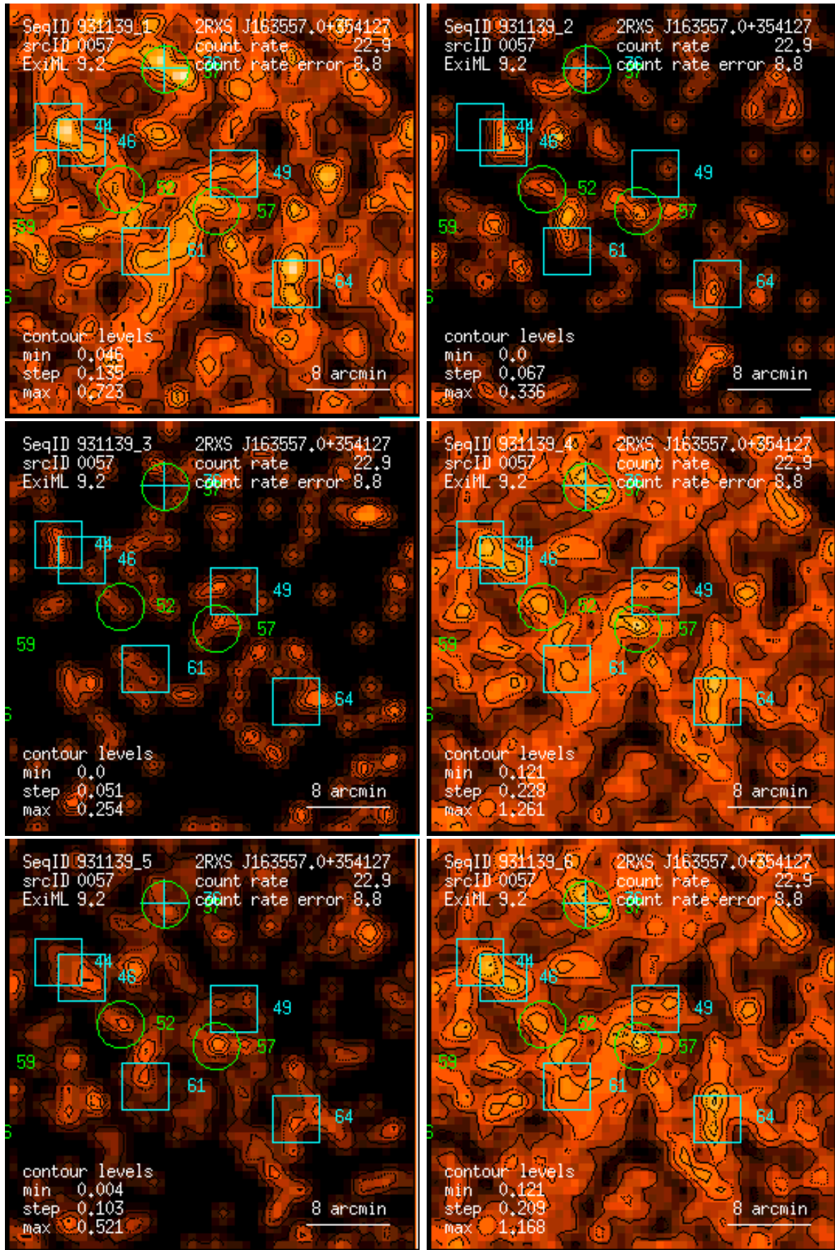
Figure 57: RASS 931139: detection 0057: band rate images, Gaussian filter: (1) PSPC channels 11 – 41, (2) 52 – 90, (3) 91 – 201, (4) 11 – 235, (5) 52 – 201, (6) 11 – 201. Broad band rates in counts/ks. Band rate contour levels in counts/ks/arcmin 2 .
