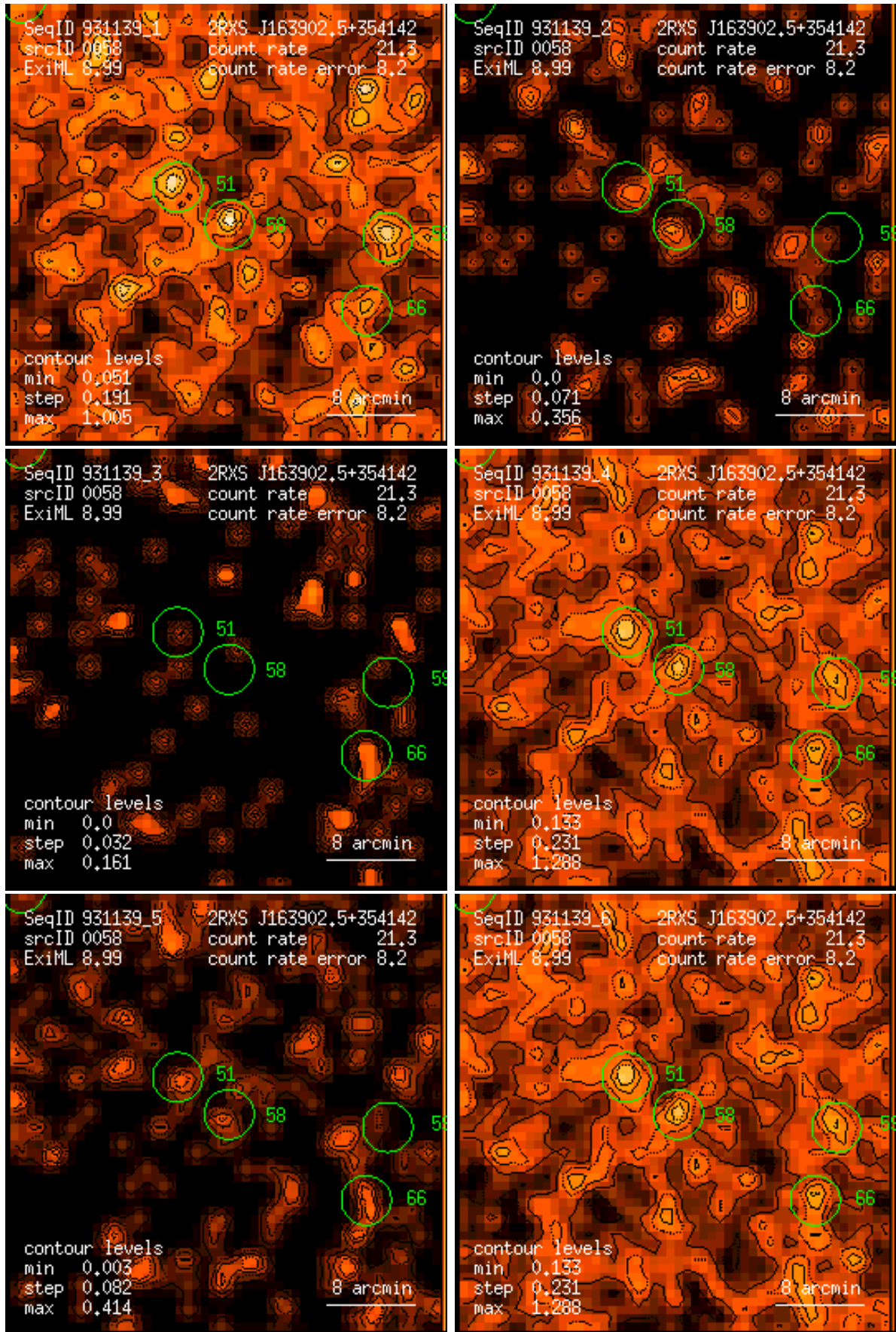
Figure 58: RASS 931139: detection 0058: band rate images, Gaussian filter: (1) PSPC channels 11 – 41, (2) 52 – 90, (3) 91 – 201, (4) 11 – 235, (5) 52 – 201, (6) 11 – 201. Broad band rates in counts/ks. Band rate contour levels in counts/ks/arcmin 2 .
