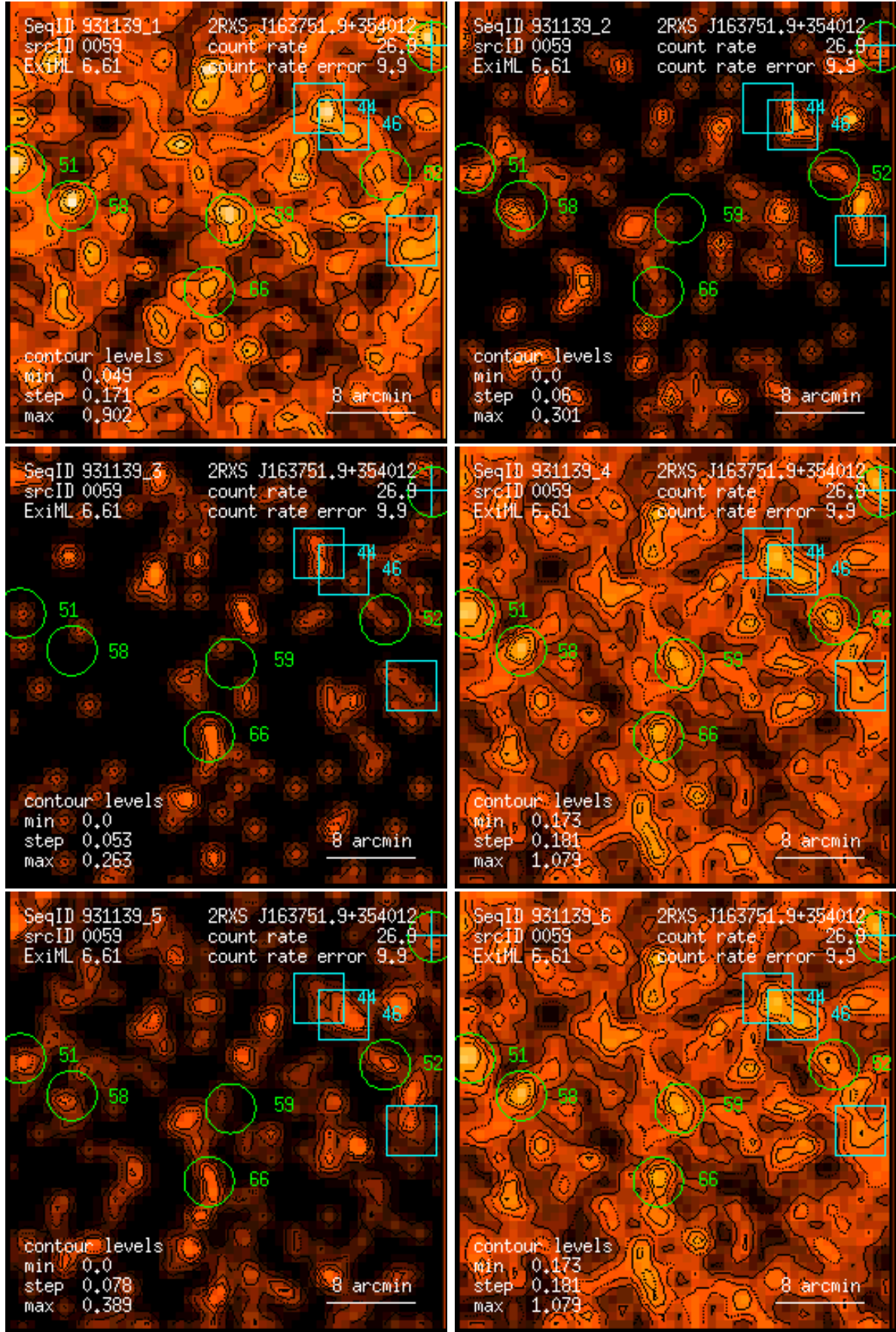
Figure 59: RASS 931139: detection 0059: band rate images, Gaussian filter: (1) PSPC channels 11 – 41, (2) 52 – 90, (3) 91 – 201, (4) 11 – 235, (5) 52 – 201, (6) 11 – 201. Broad band rates in counts/ks. Band rate contour levels in counts/ks/arcmin 2 .
