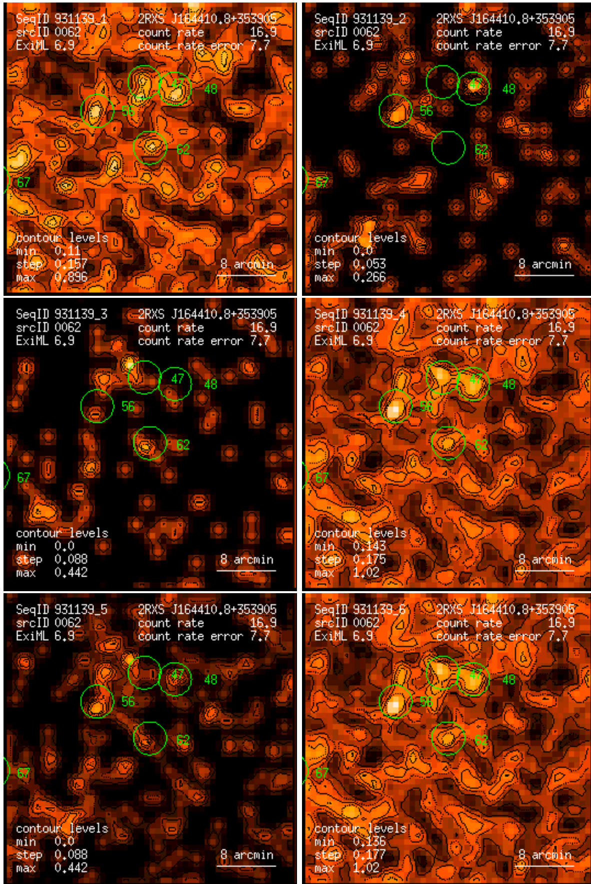
Figure 62: RASS 931139: detection 0062: band rate images, Gaussian filter: (1) PSPC channels 11 – 41, (2) 52 – 90, (3) 91 – 201, (4) 11 – 235, (5) 52 – 201, (6) 11 – 201. Broad band rates in counts/ks. Band rate contour levels in counts/ks/arcmin 2 .
