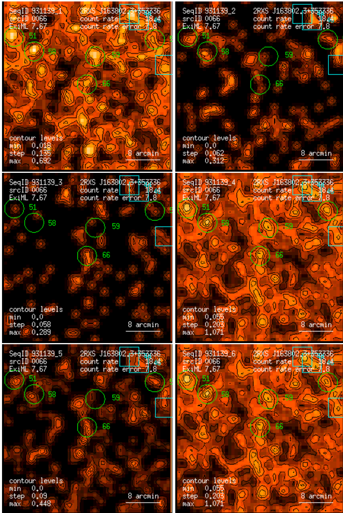
Figure 66: RASS 931139: detection 0066: band rate images, Gaussian filter: (1) PSPC channels 11 – 41, (2) 52 – 90, (3) 91 – 201, (4) 11 – 235, (5) 52 – 201, (6) 11 – 201. Broad band rates in counts/ks. Band rate contour levels in counts/ks/arcmin 2 .
