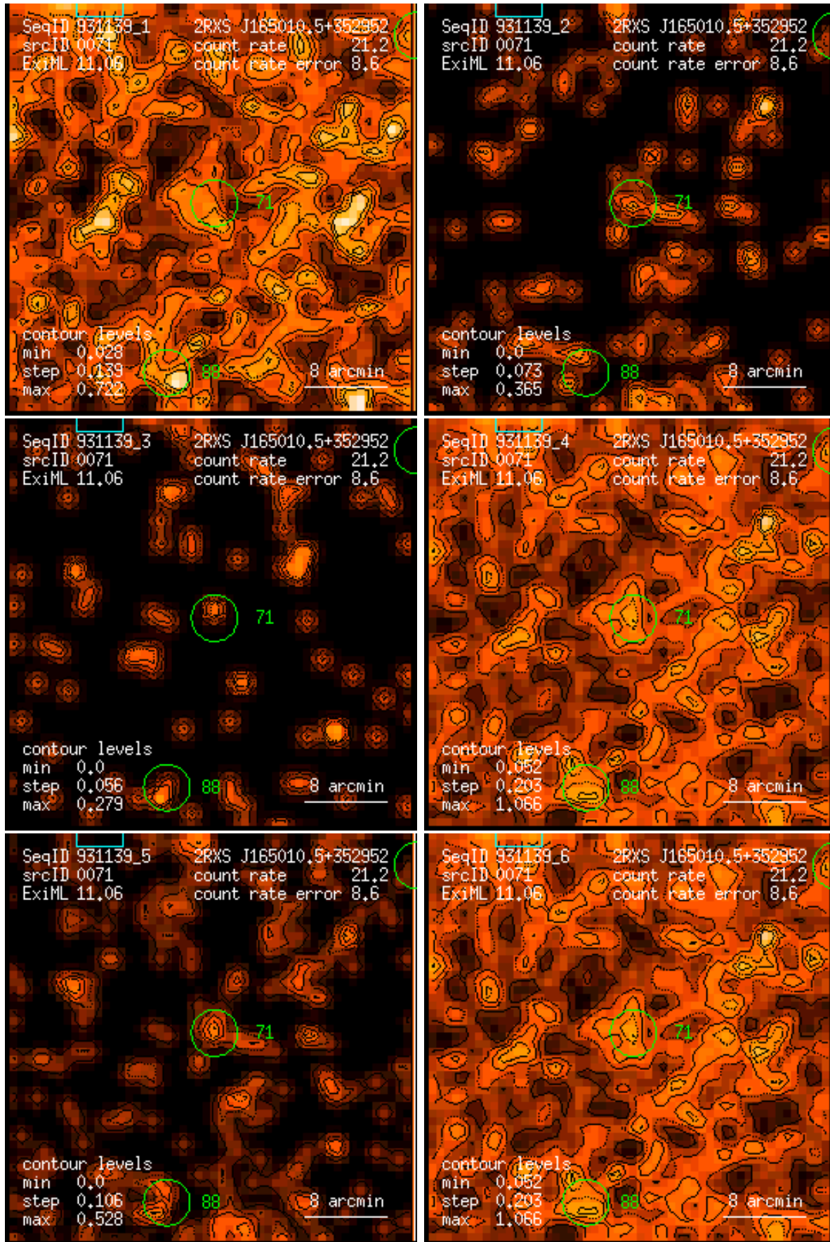
Figure 71: RASS 931139: detection 0071: band rate images, Gaussian filter: (1) PSPC channels 11 – 41, (2) 52 – 90, (3) 91 – 201, (4) 11 – 235, (5) 52 – 201, (6) 11 – 201. Broad band rates in counts/ks. Band rate contour levels in counts/ks/arcmin 2 .
