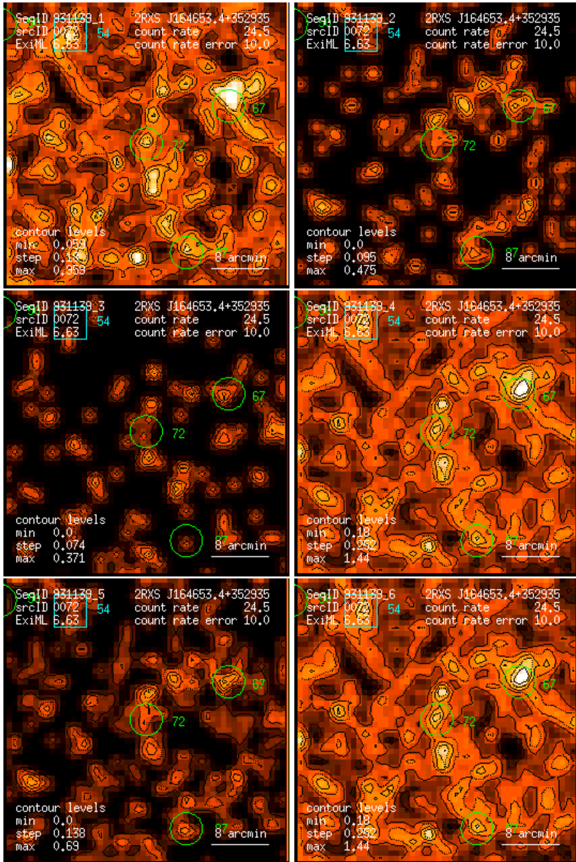
Figure 72: RASS 931139: detection 0072: band rate images, Gaussian filter: (1) PSPC channels 11 – 41, (2) 52 – 90, (3) 91 – 201, (4) 11 – 235, (5) 52 – 201, (6) 11 – 201. Broad band rates in counts/ks. Band rate contour levels in counts/ks/arcmin 2 .
