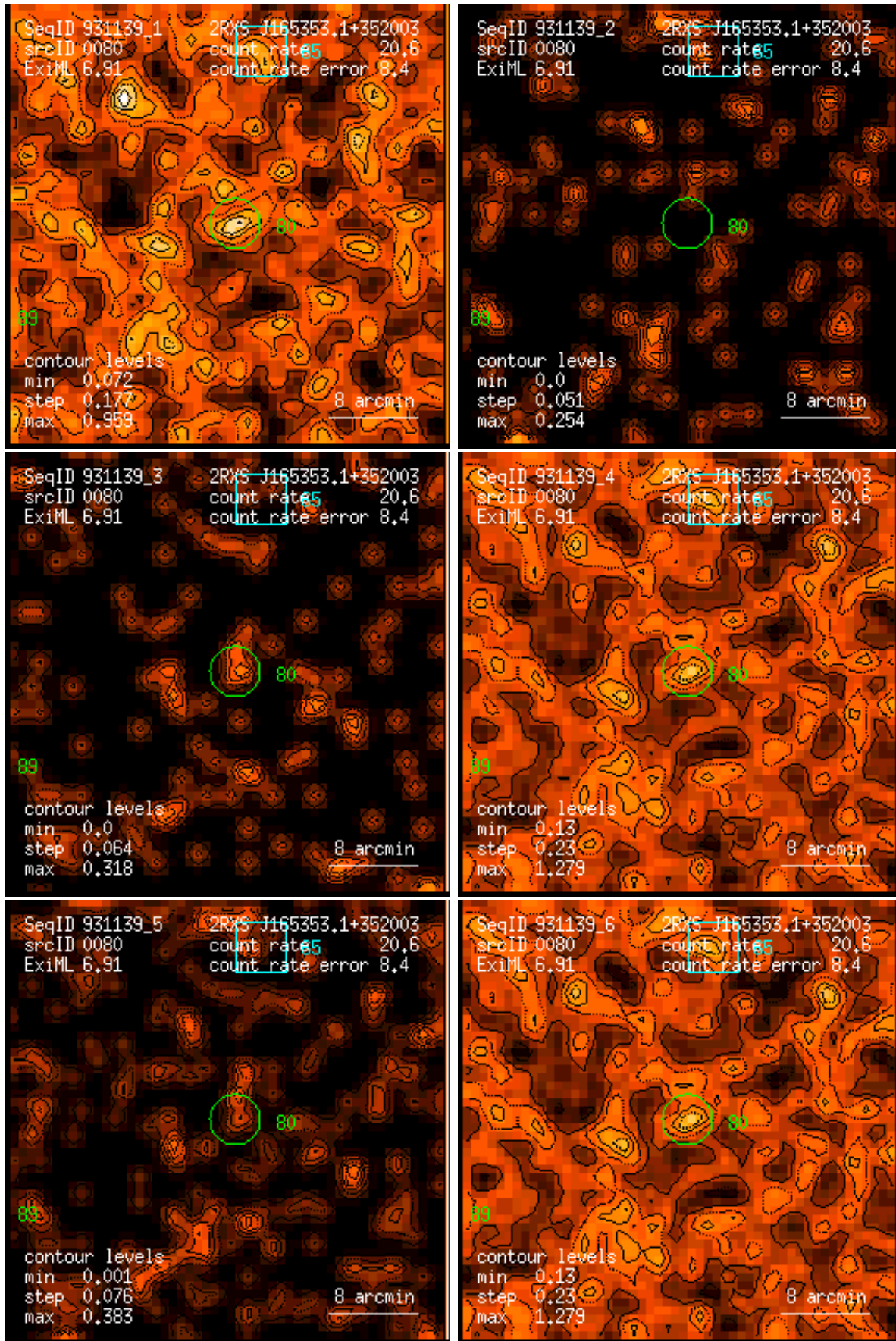
Figure 80: RASS 931139: detection 0080: band rate images, Gaussian filter: (1) PSPC channels 11 – 41, (2) 52 – 90, (3) 91 – 201, (4) 11 – 235, (5) 52 – 201, (6) 11 – 201. Broad band rates in counts/ks. Band rate contour levels in counts/ks/arcmin 2 .
