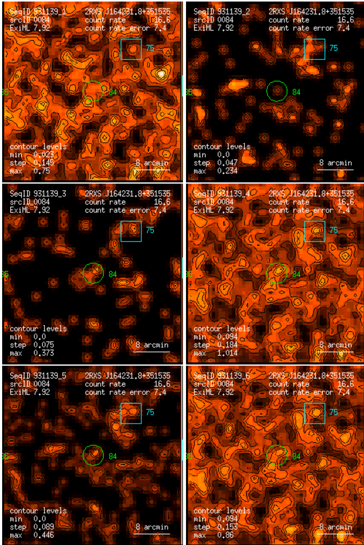
Figure 84: RASS 931139: detection 0084: band rate images, Gaussian filter: (1) PSPC channels 11 – 41, (2) 52 – 90, (3) 91 – 201, (4) 11 – 235, (5) 52 – 201, (6) 11 – 201. Broad band rates in counts/ks. Band rate contour levels in counts/ks/arcmin 2 .
