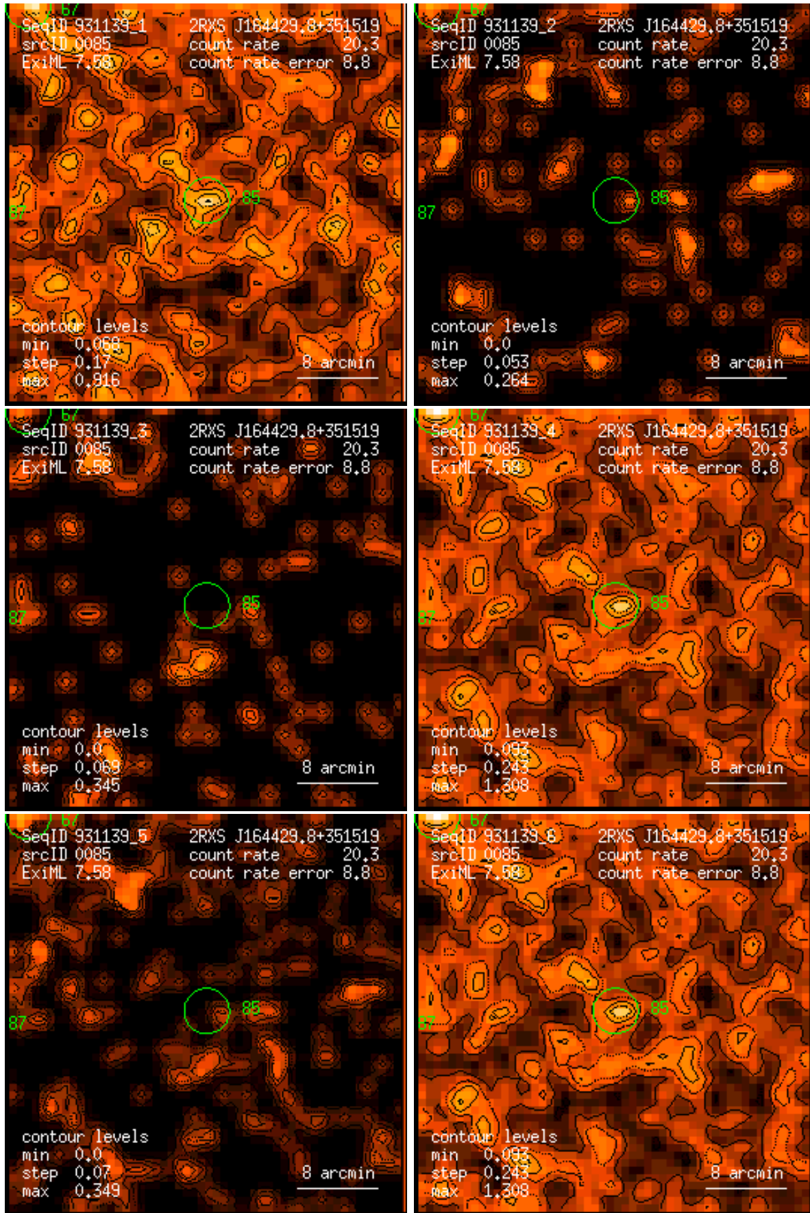
Figure 85: RASS 931139: detection 0085: band rate images, Gaussian filter: (1) PSPC channels 11 – 41, (2) 52 – 90, (3) 91 – 201, (4) 11 – 235, (5) 52 – 201, (6) 11 – 201. Broad band rates in counts/ks. Band rate contour levels in counts/ks/arcmin 2 .
