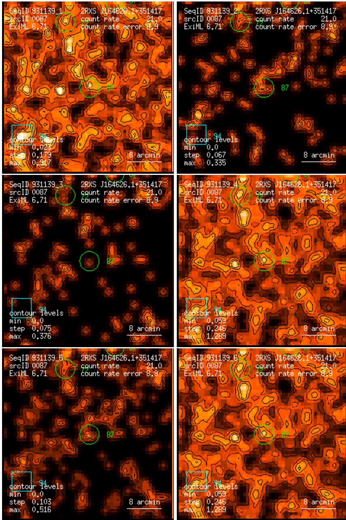
Figure 87: RASS 931139: detection 0087: band rate images, Gaussian filter: (1) PSPC channels 11 – 41, (2) 52 – 90, (3) 91 – 201, (4) 11 – 235, (5) 52 – 201, (6) 11 – 201. Broad band rates in counts/ks. Band rate contour levels in counts/ks/arcmin 2 .
