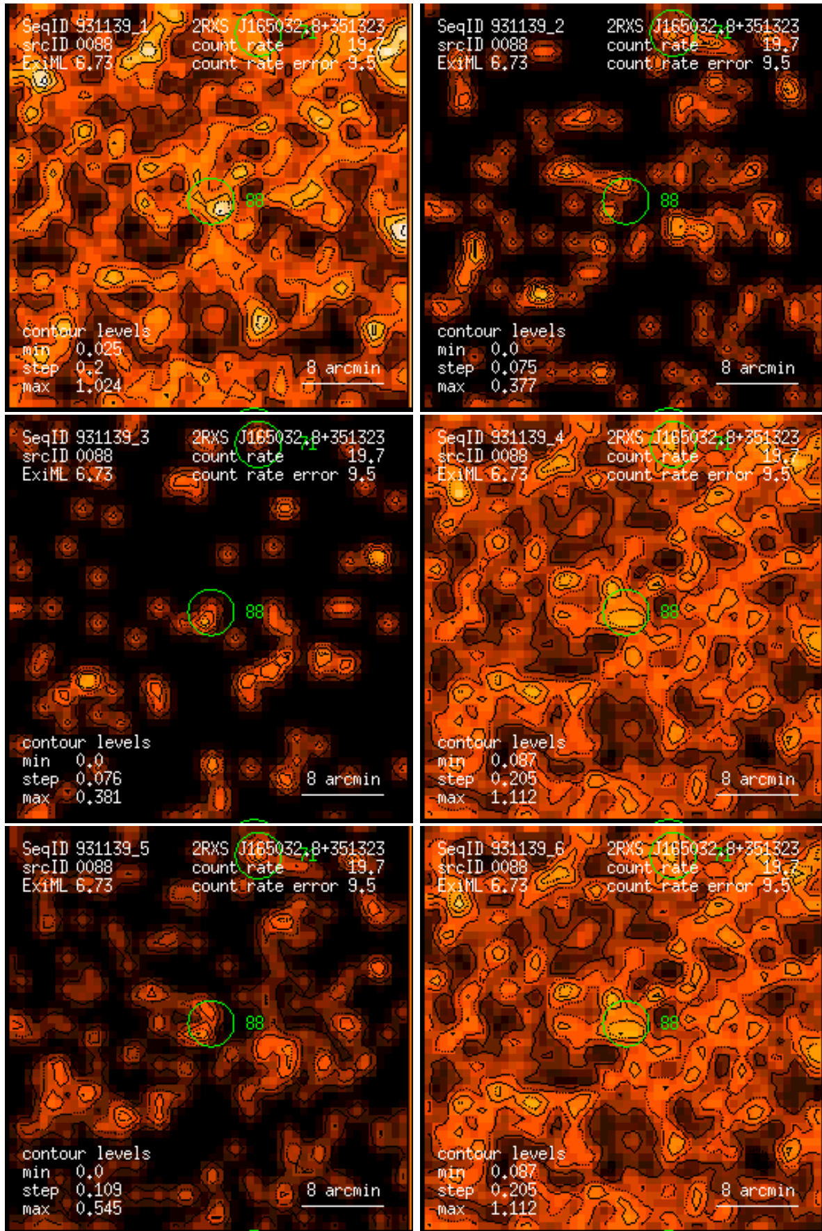
Figure 88: RASS 931139: detection 0088: band rate images, Gaussian filter: (1) PSPC channels 11 – 41, (2) 52 – 90, (3) 91 – 201, (4) 11 – 235, (5) 52 – 201, (6) 11 – 201. Broad band rates in counts/ks. Band rate contour levels in counts/ks/arcmin 2 .
