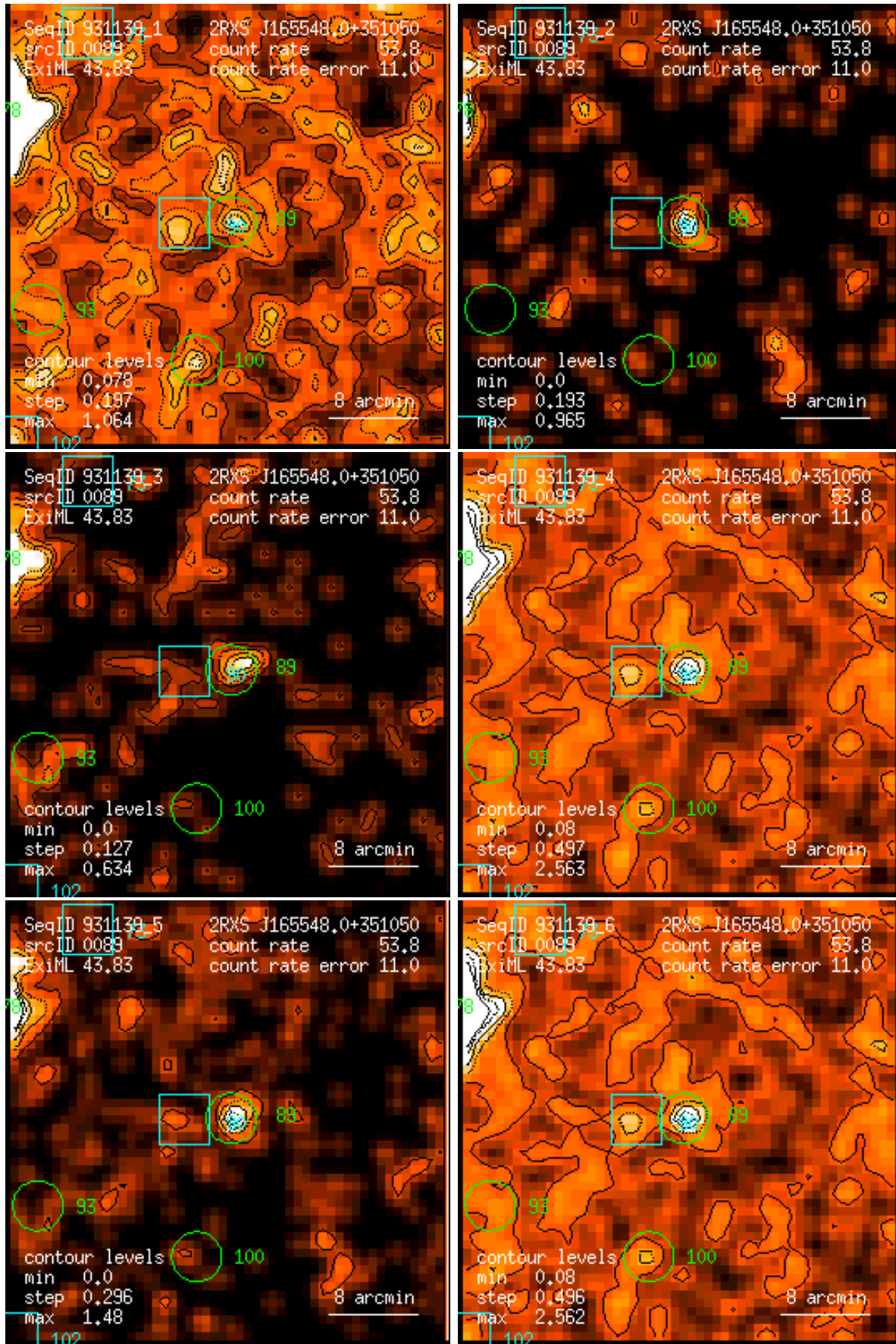
Figure 89: RASS 931139: detection 0089: band rate images, Gaussian filter: (1) PSPC channels 11 – 41, (2) 52 – 90, (3) 91 – 201, (4) 11 – 235, (5) 52 – 201, (6) 11 – 201. Broad band rates in counts/ks. Band rate contour levels in counts/ks/arcmin 2 .
