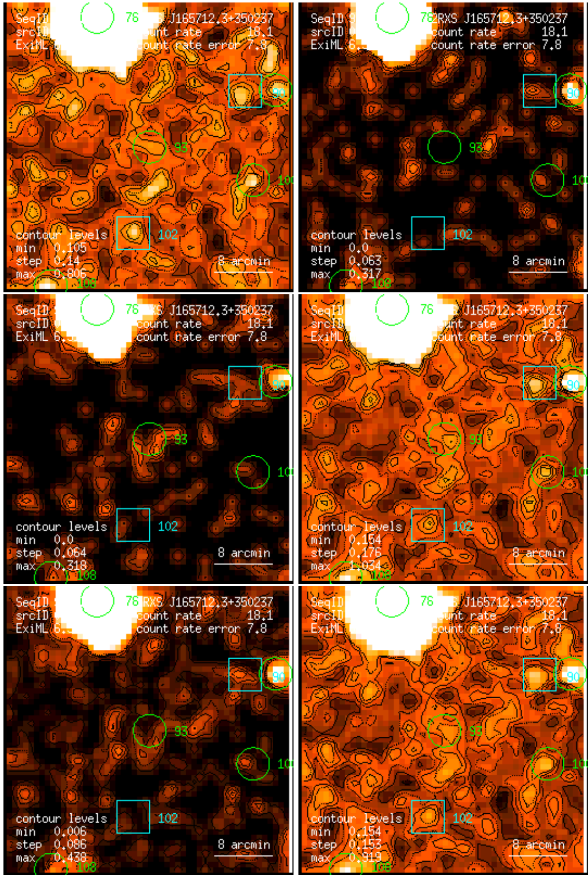
Figure 93: RASS 931139: detection 0093: band rate images, Gaussian filter: (1) PSPC channels 11 – 41, (2) 52 – 90, (3) 91 – 201, (4) 11 – 235, (5) 52 – 201, (6) 11 – 201. Broad band rates in counts/ks. Band rate contour levels in counts/ks/arcmin 2 .
