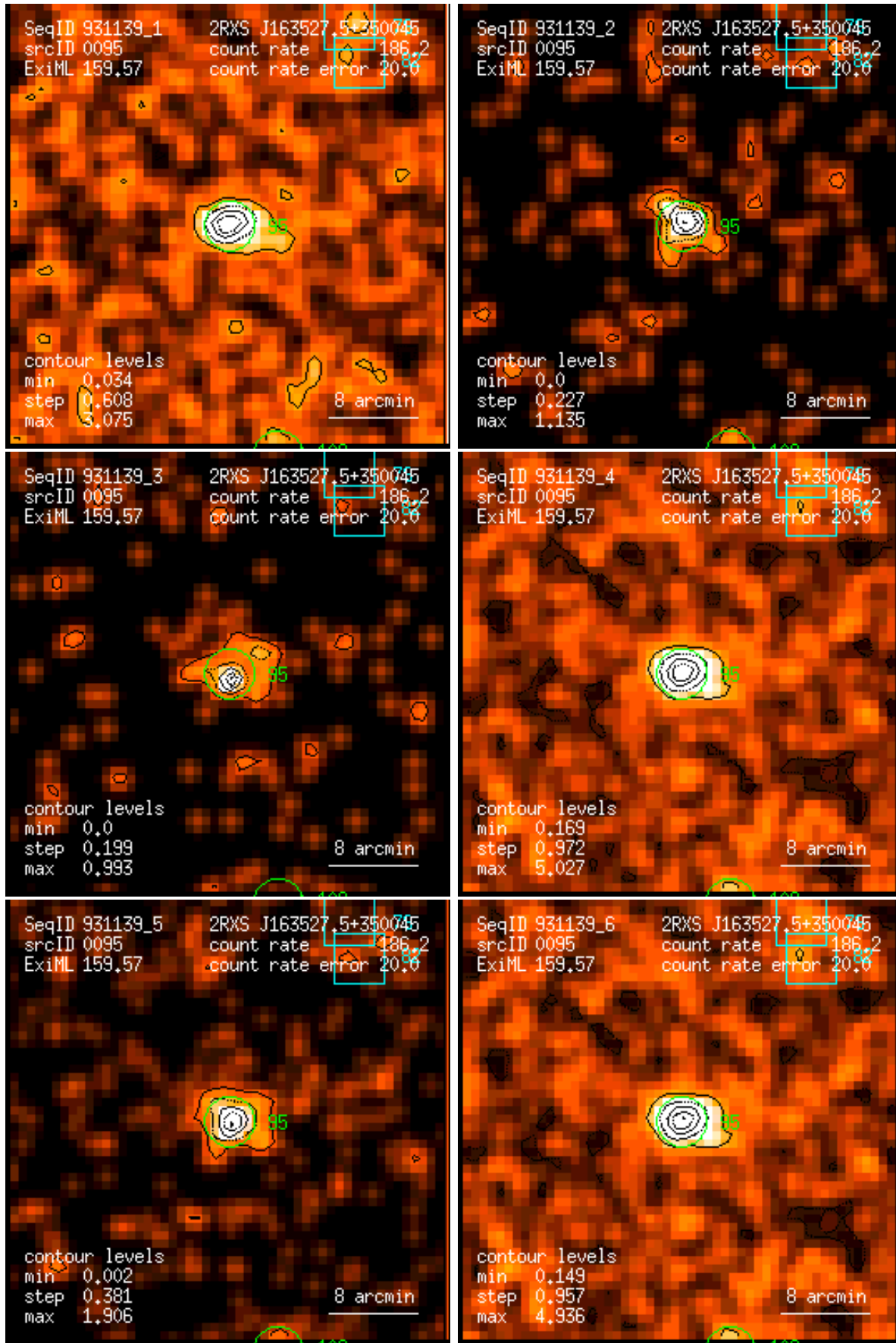
Figure 95: RASS 931139: detection 0095: band rate images, Gaussian filter: (1) PSPC channels 11 – 41, (2) 52 – 90, (3) 91 – 201, (4) 11 – 235, (5) 52 – 201, (6) 11 – 201. Broad band rates in counts/ks. Band rate contour levels in counts/ks/arcmin 2 .
