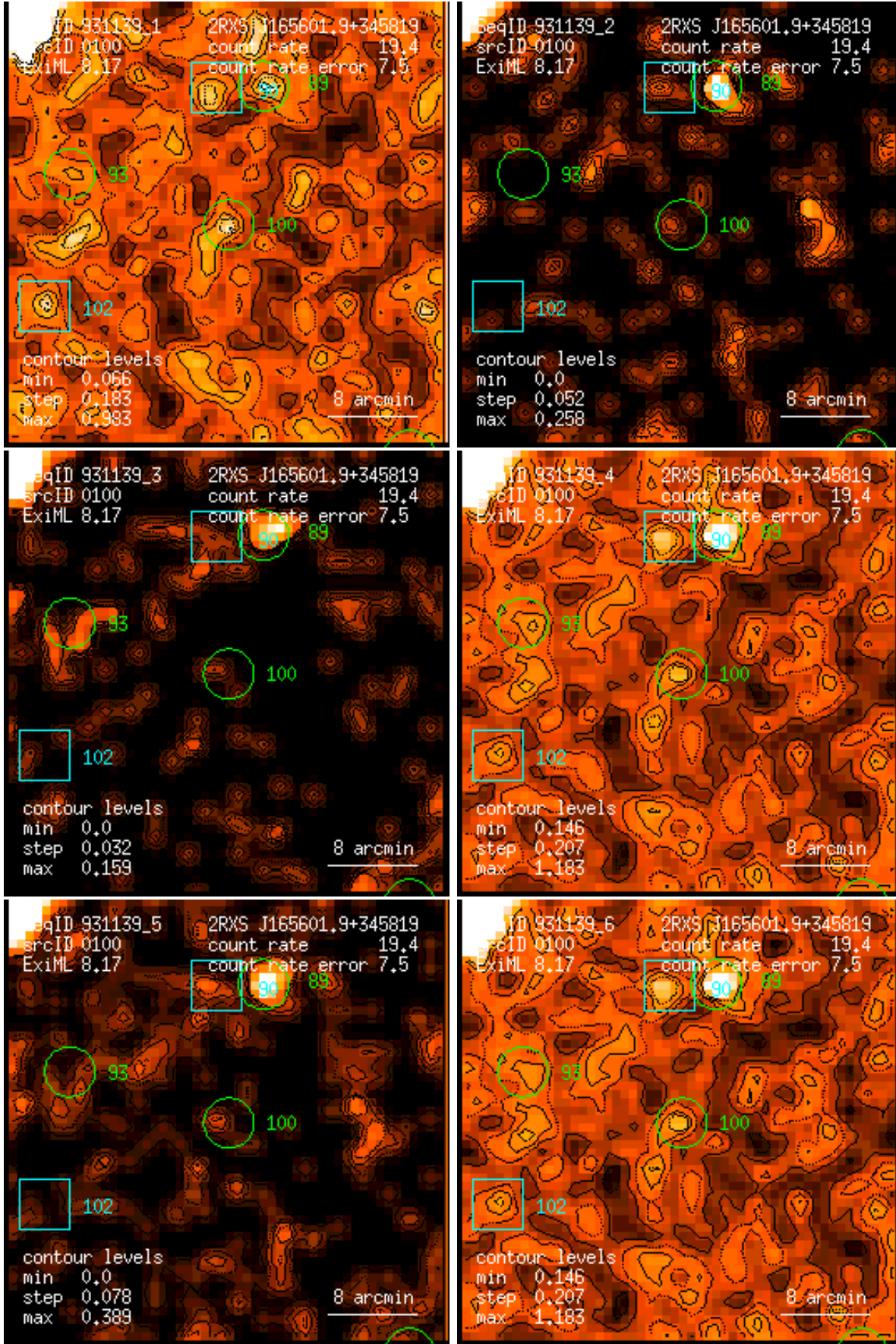
Figure 100: RASS 931139: detection 0100: band rate images, Gaussian filter: (1) PSPC channels 11 – 41, (2) 52 – 90, (3) 91 – 201, (4) 11 – 235, (5) 52 – 201, (6) 11 – 201. Broad band rates in counts/ks. Band rate contour levels in counts/ks/arcmin 2 .
