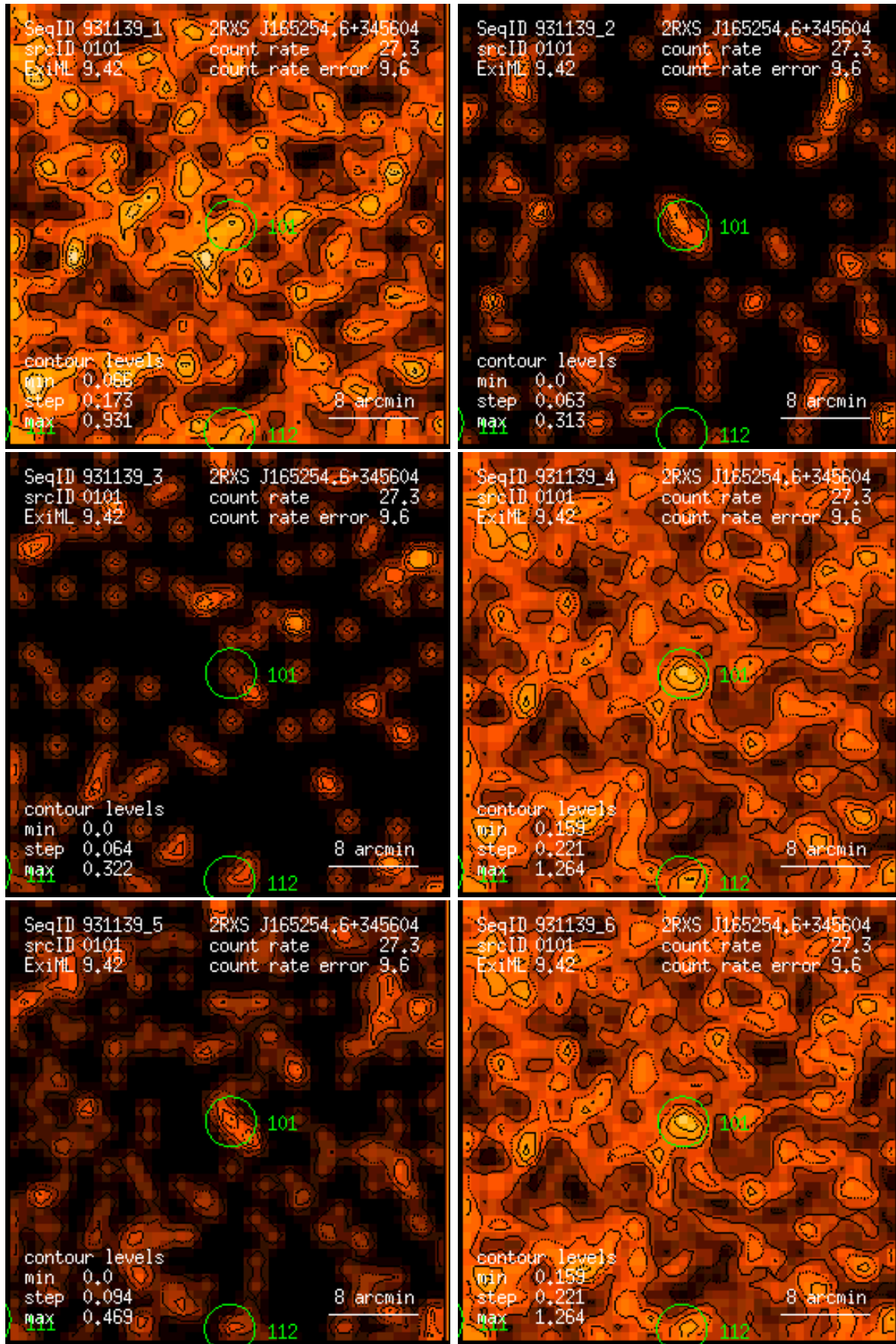
Figure 101: RASS 931139: detection 0101: band rate images, Gaussian filter: (1) PSPC channels 11 – 41, (2) 52 – 90, (3) 91 – 201, (4) 11 – 235, (5) 52 – 201, (6) 11 – 201. Broad band rates in counts/ks. Band rate contour levels in counts/ks/arcmin 2 .
