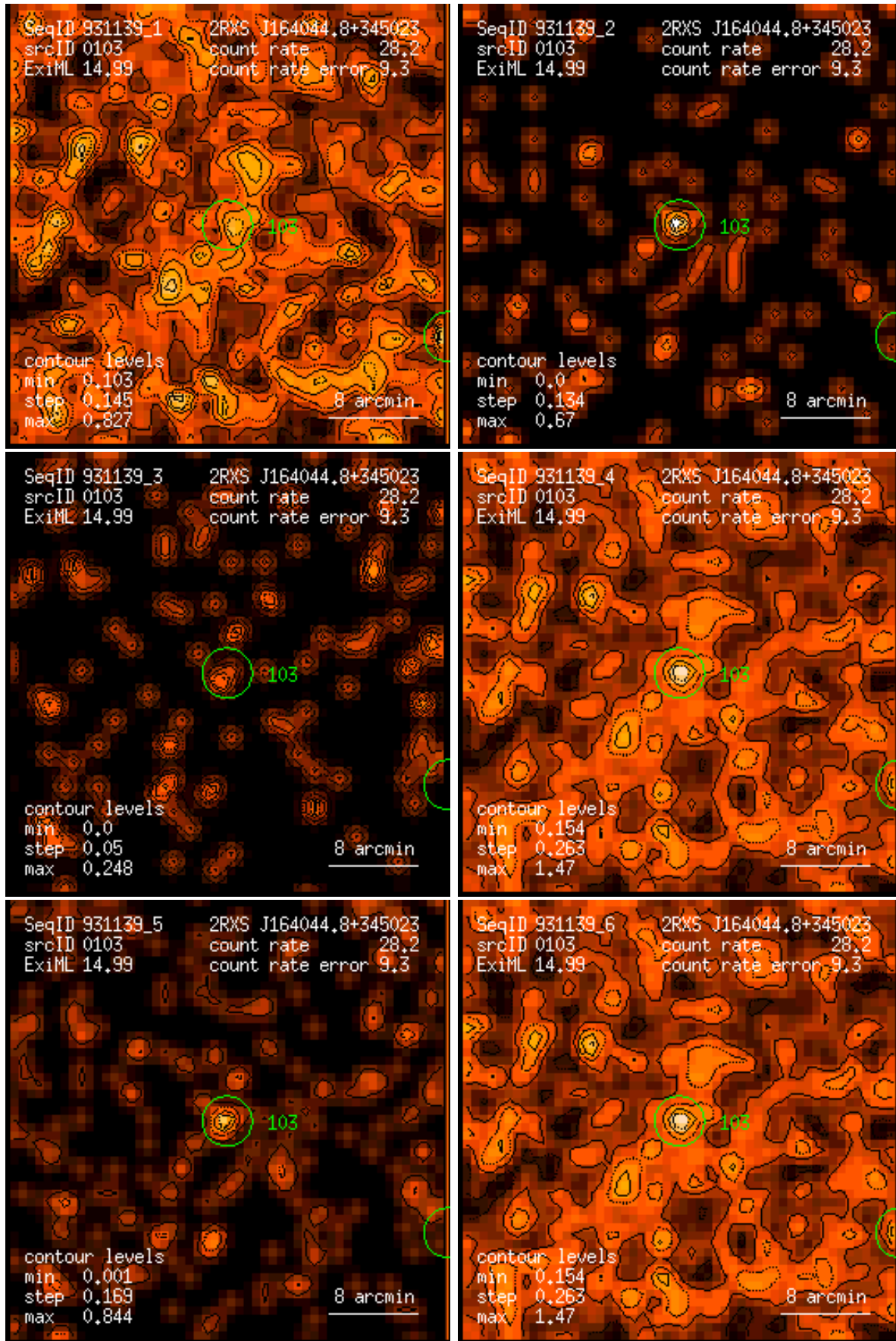
Figure 103: RASS 931139: detection 0103: band rate images, Gaussian filter: (1) PSPC channels 11 – 41, (2) 52 – 90, (3) 91 – 201, (4) 11 – 235, (5) 52 – 201, (6) 11 – 201. Broad band rates in counts/ks. Band rate contour levels in counts/ks/arcmin 2 .
