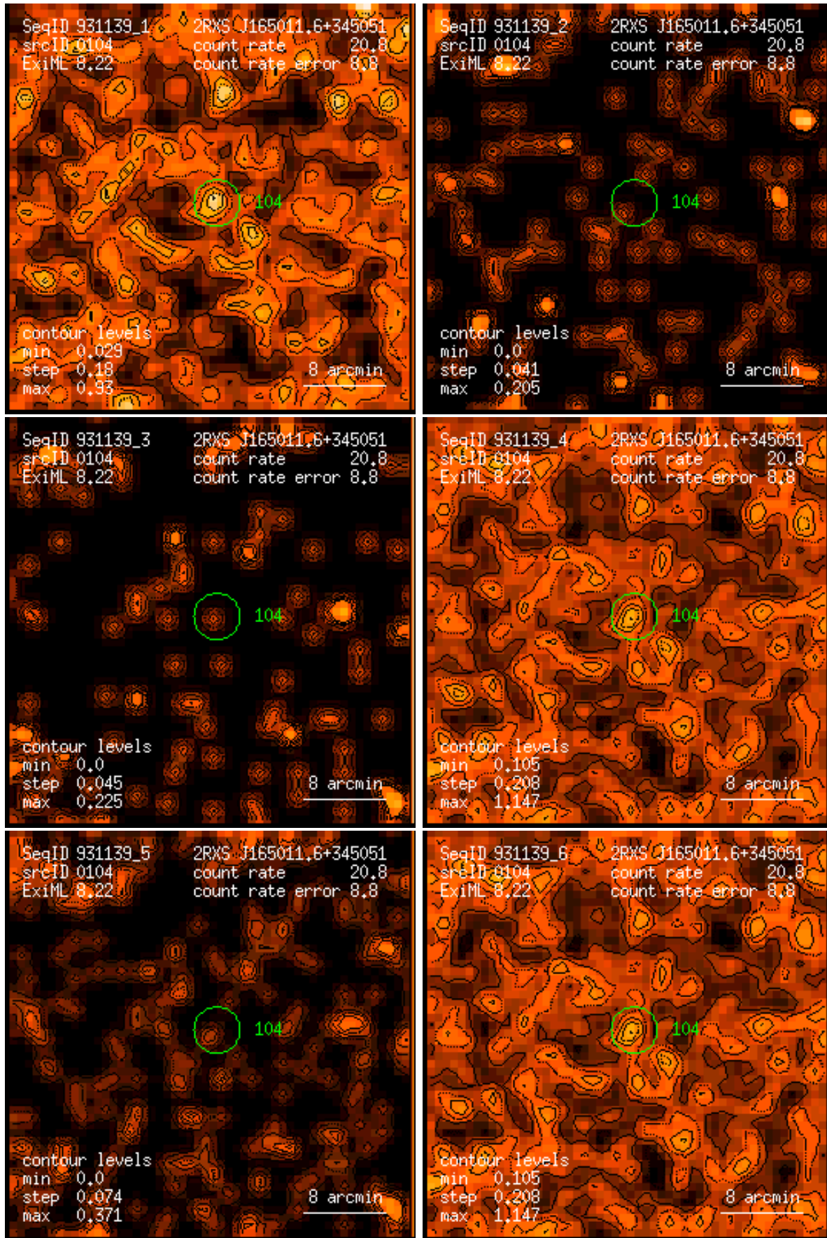
Figure 104: RASS 931139: detection 0104: band rate images, Gaussian filter: (1) PSPC channels 11 – 41, (2) 52 – 90, (3) 91 – 201, (4) 11 – 235, (5) 52 – 201, (6) 11 – 201. Broad band rates in counts/ks. Band rate contour levels in counts/ks/arcmin 2 .
