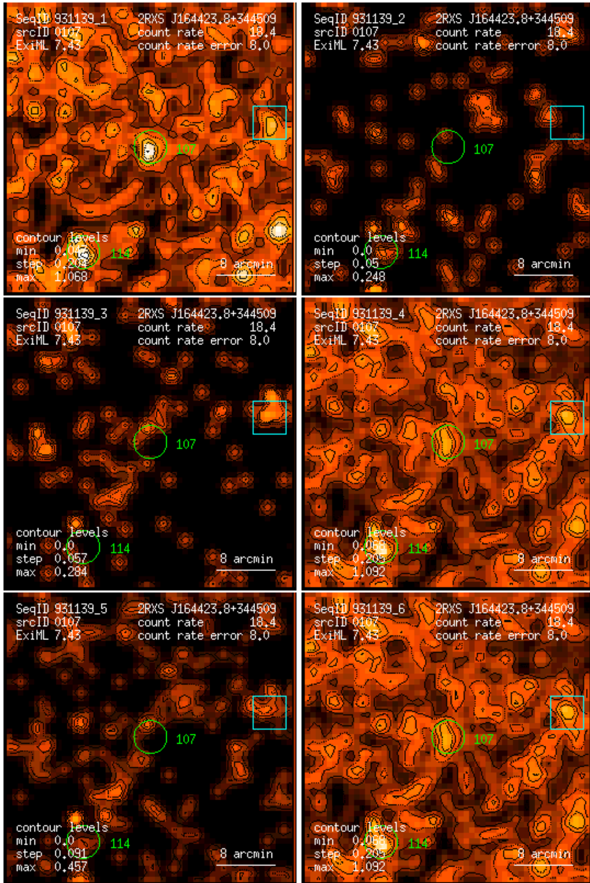
Figure 107: RASS 931139: detection 0107: band rate images, Gaussian filter: (1) PSPC channels 11 – 41, (2) 52 – 90, (3) 91 – 201, (4) 11 – 235, (5) 52 – 201, (6) 11 – 201. Broad band rates in counts/ks. Band rate contour levels in counts/ks/arcmin 2 .
