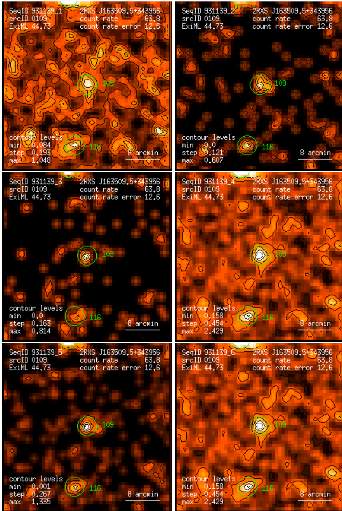
Figure 109: RASS 931139: detection 0109: band rate images, Gaussian filter: (1) PSPC channels 11 – 41, (2) 52 – 90, (3) 91 – 201, (4) 11 – 235, (5) 52 – 201, (6) 11 – 201. Broad band rates in counts/ks. Band rate contour levels in counts/ks/arcmin 2 .
