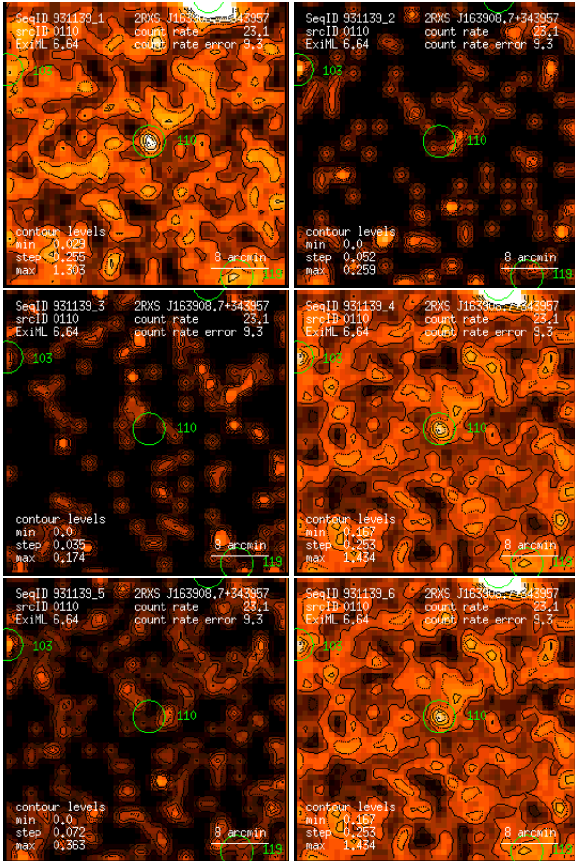
Figure 110: RASS 931139: detection 0110: band rate images, Gaussian filter: (1) PSPC channels 11 – 41, (2) 52 – 90, (3) 91 – 201, (4) 11 – 235, (5) 52 – 201, (6) 11 – 201. Broad band rates in counts/ks. Band rate contour levels in counts/ks/arcmin 2 .
