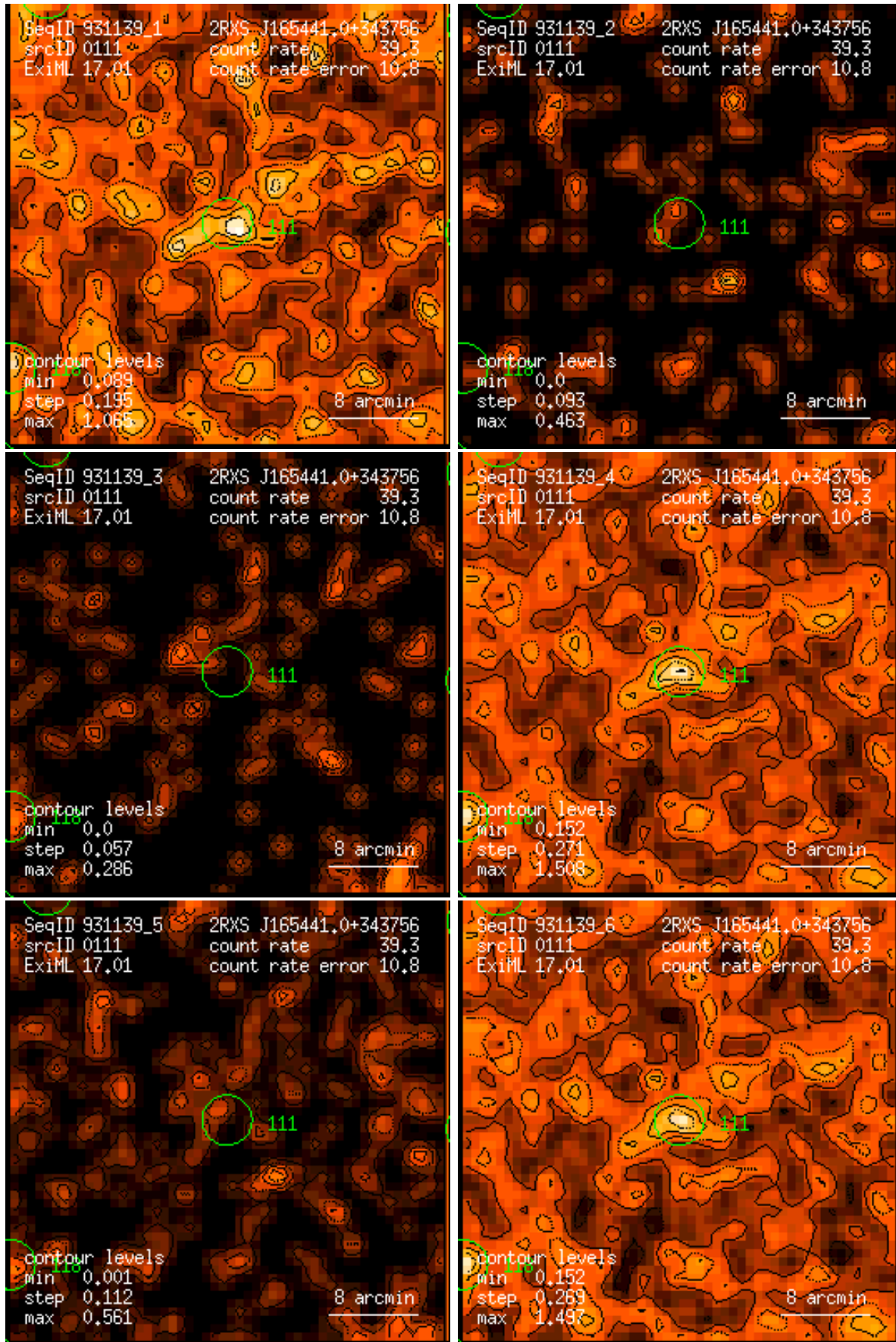
Figure 111: RASS 931139: detection 0111: band rate images, Gaussian filter: (1) PSPC channels 11 – 41, (2) 52 – 90, (3) 91 – 201, (4) 11 – 235, (5) 52 – 201, (6) 11 – 201. Broad band rates in counts/ks. Band rate contour levels in counts/ks/arcmin 2 .
