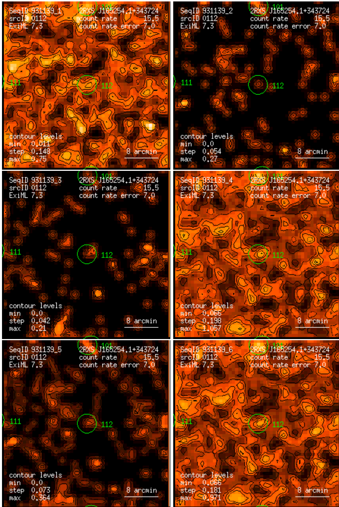
Figure 112: RASS 931139: detection 0112: band rate images, Gaussian filter: (1) PSPC channels 11 – 41, (2) 52 – 90, (3) 91 – 201, (4) 11 – 235, (5) 52 – 201, (6) 11 – 201. Broad band rates in counts/ks. Band rate contour levels in counts/ks/arcmin 2 .
