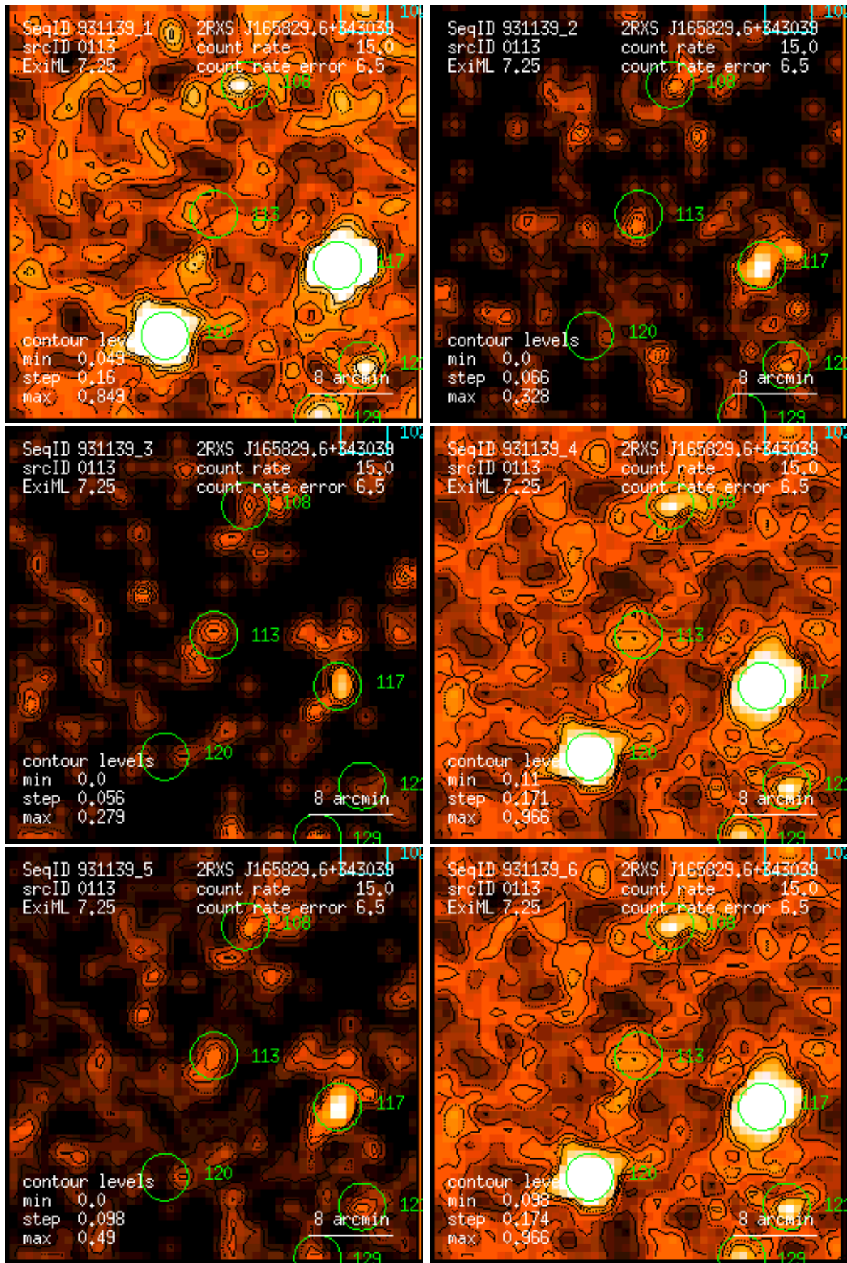
Figure 113: RASS 931139: detection 0113: band rate images, Gaussian filter: (1) PSPC channels 11 – 41, (2) 52 – 90, (3) 91 – 201, (4) 11 – 235, (5) 52 – 201, (6) 11 – 201. Broad band rates in counts/ks. Band rate contour levels in counts/ks/arcmin 2 .
