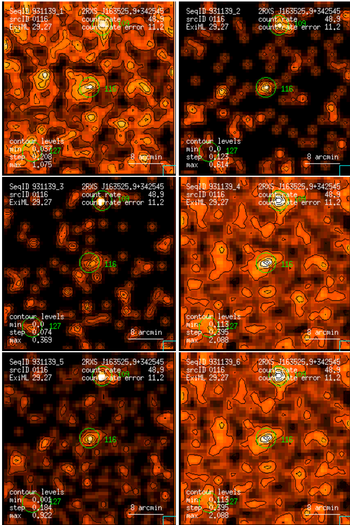
Figure 116: RASS 931139: detection 0116: band rate images, Gaussian filter: (1) PSPC channels 11 – 41, (2) 52 – 90, (3) 91 – 201, (4) 11 – 235, (5) 52 – 201, (6) 11 – 201. Broad band rates in counts/ks. Band rate contour levels in counts/ks/arcmin 2 .
