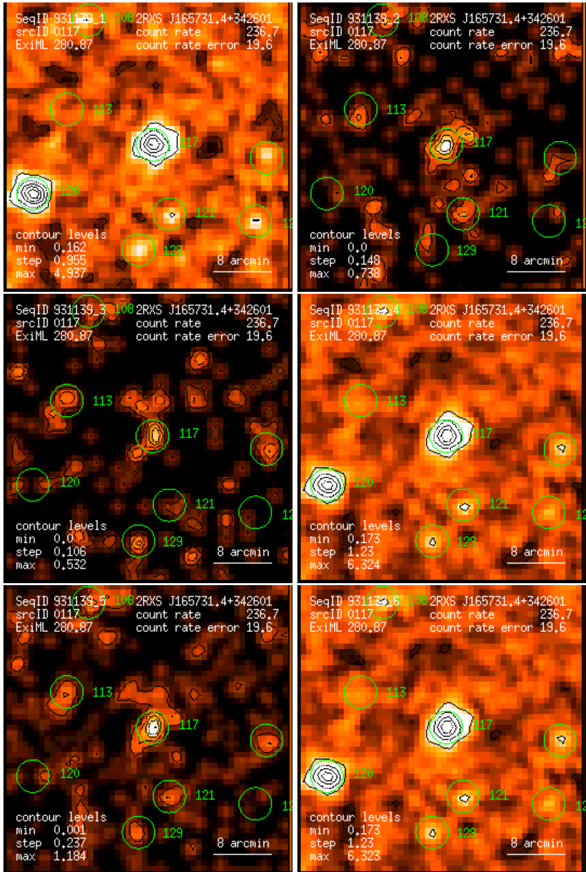
Figure 117: RASS 931139: detection 0117: band rate images, Gaussian filter: (1) PSPC channels 11 – 41, (2) 52 – 90, (3) 91 – 201, (4) 11 – 235, (5) 52 – 201, (6) 11 – 201. Broad band rates in counts/ks. Band rate contour levels in counts/ks/arcmin 2 .
