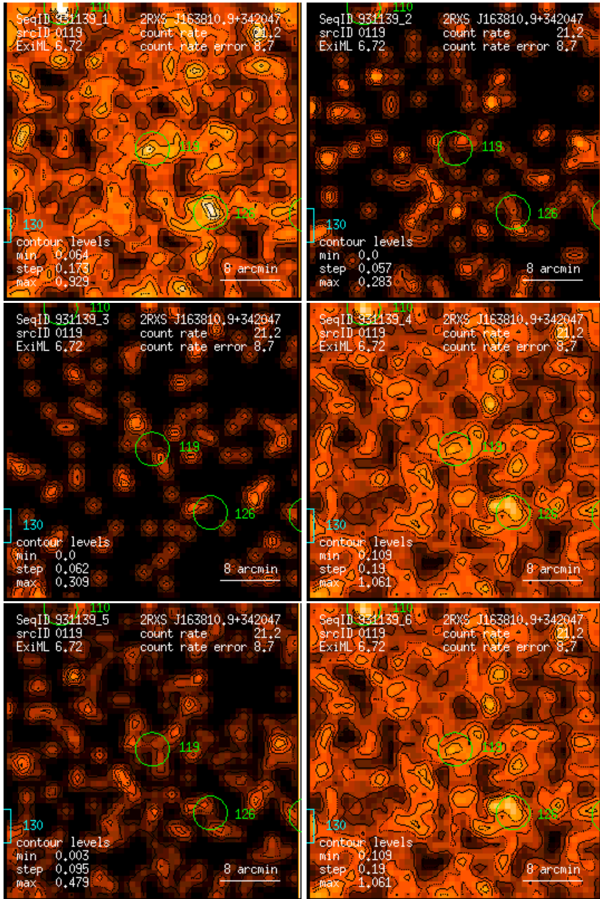
Figure 119: RASS 931139: detection 0119: band rate images, Gaussian filter: (1) PSPC channels 11 – 41, (2) 52 – 90, (3) 91 – 201, (4) 11 – 235, (5) 52 – 201, (6) 11 – 201. Broad band rates in counts/ks. Band rate contour levels in counts/ks/arcmin 2 .
