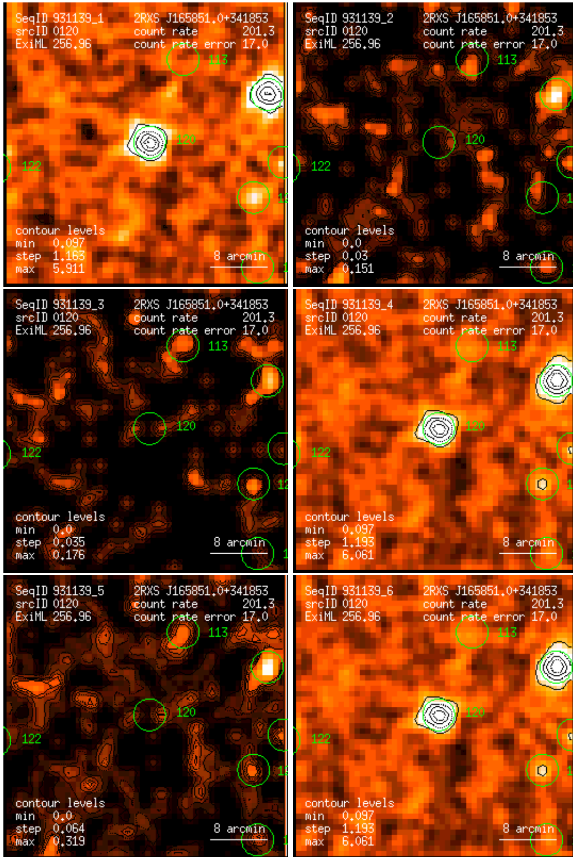
Figure 120: RASS 931139: detection 0120: band rate images, Gaussian filter: (1) PSPC channels 11 – 41, (2) 52 – 90, (3) 91 – 201, (4) 11 – 235, (5) 52 – 201, (6) 11 – 201. Broad band rates in counts/ks. Band rate contour levels in counts/ks/arcmin 2 .
