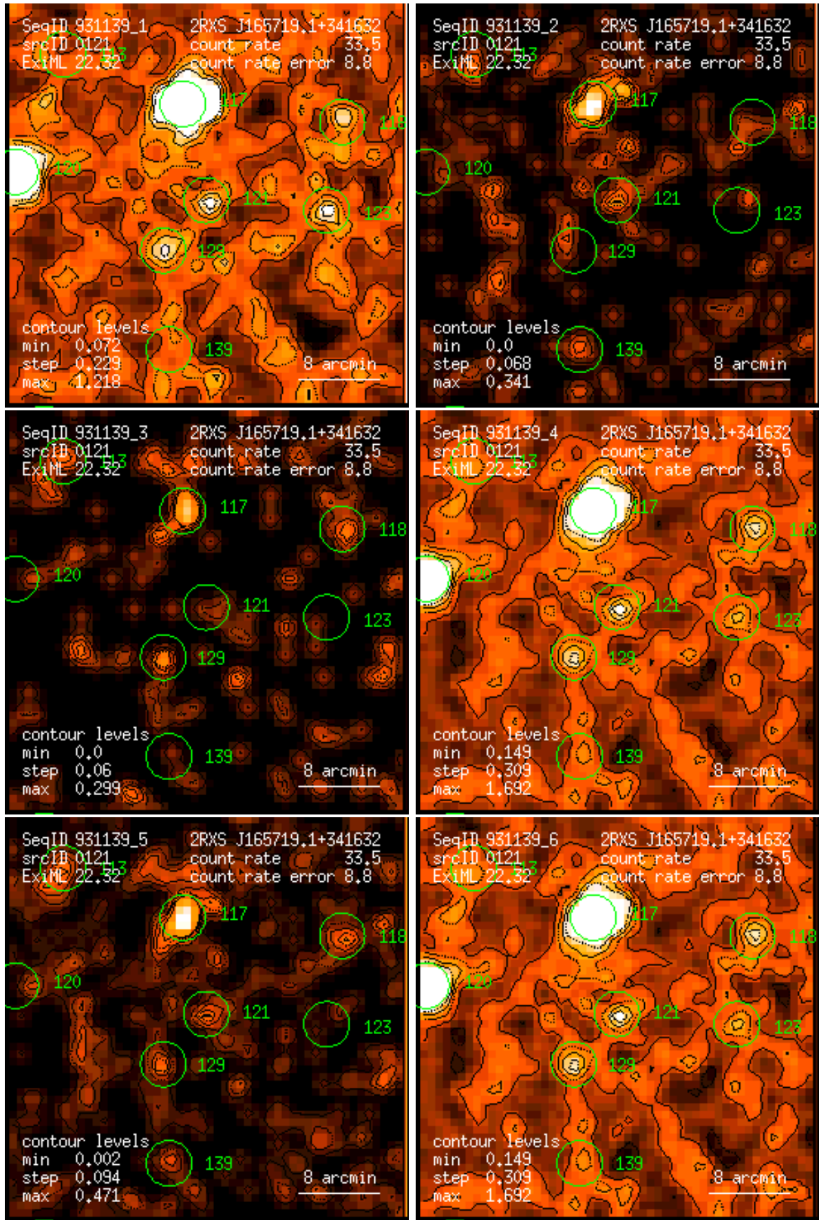
Figure 121: RASS 931139: detection 0121: band rate images, Gaussian filter: (1) PSPC channels 11 – 41, (2) 52 – 90, (3) 91 – 201, (4) 11 – 235, (5) 52 – 201, (6) 11 – 201. Broad band rates in counts/ks. Band rate contour levels in counts/ks/arcmin 2 .
