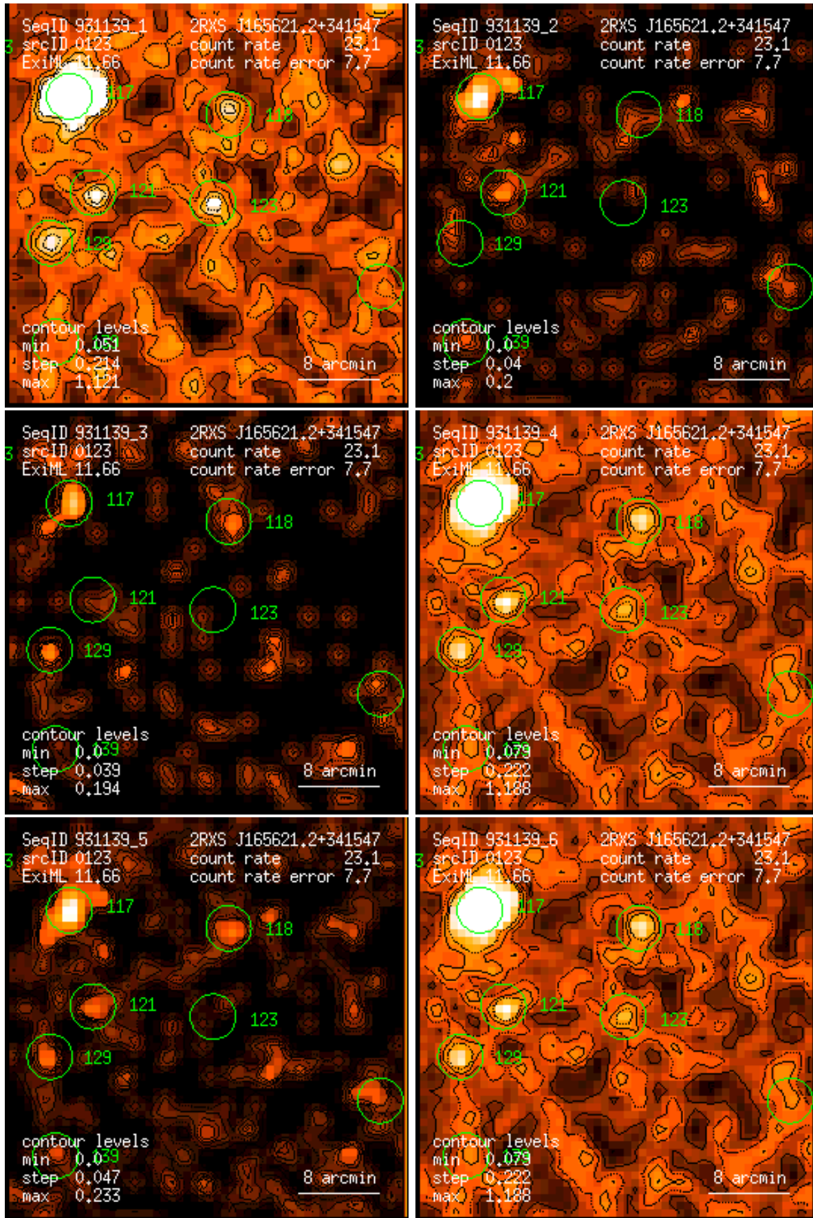
Figure 123: RASS 931139: detection 0123: band rate images, Gaussian filter: (1) PSPC channels 11 – 41, (2) 52 – 90, (3) 91 – 201, (4) 11 – 235, (5) 52 – 201, (6) 11 – 201. Broad band rates in counts/ks. Band rate contour levels in counts/ks/arcmin 2 .
