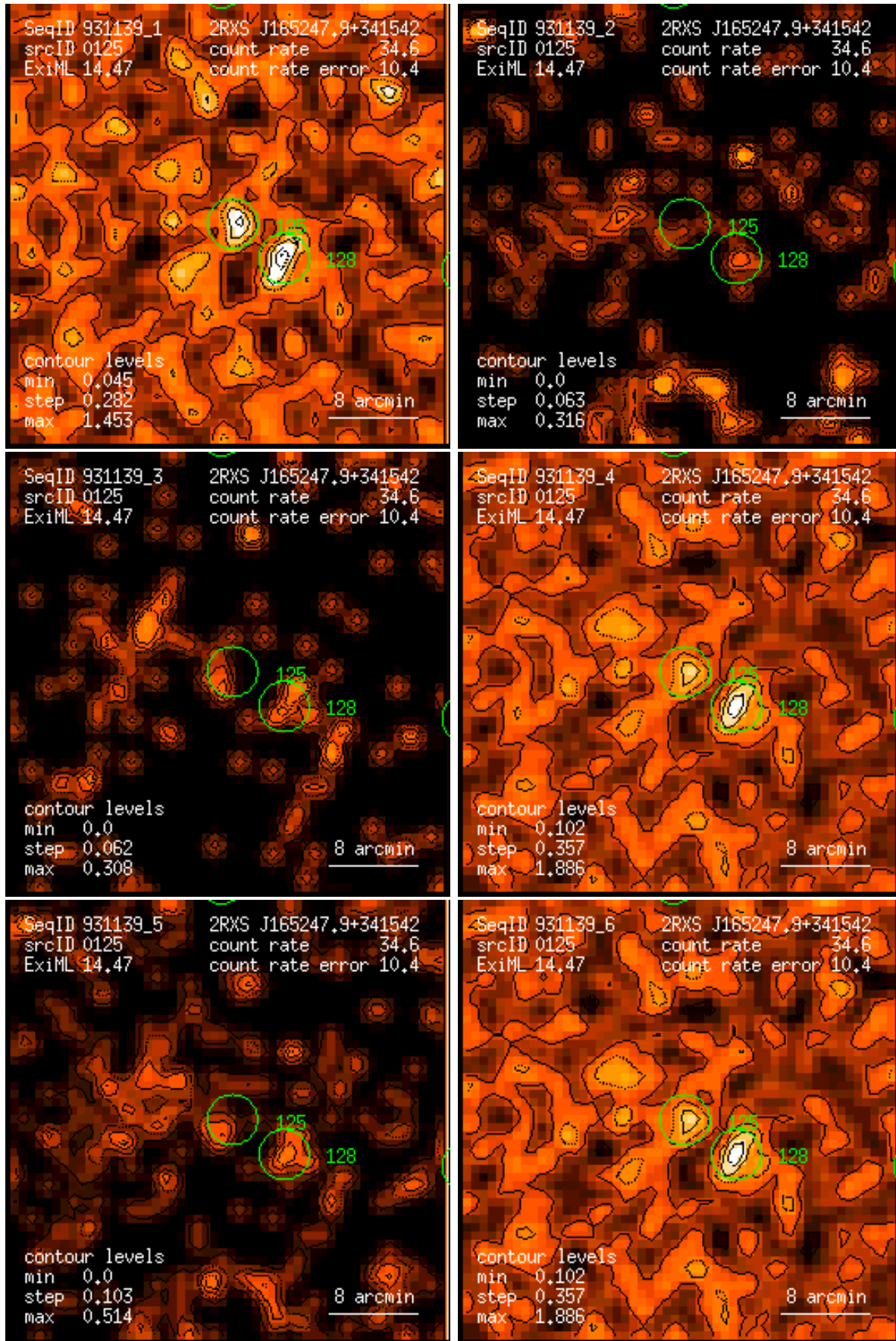
Figure 125: RASS 931139: detection 0125: band rate images, Gaussian filter: (1) PSPC channels 11 – 41, (2) 52 – 90, (3) 91 – 201, (4) 11 – 235, (5) 52 – 201, (6) 11 – 201. Broad band rates in counts/ks. Band rate contour levels in counts/ks/arcmin 2 .
