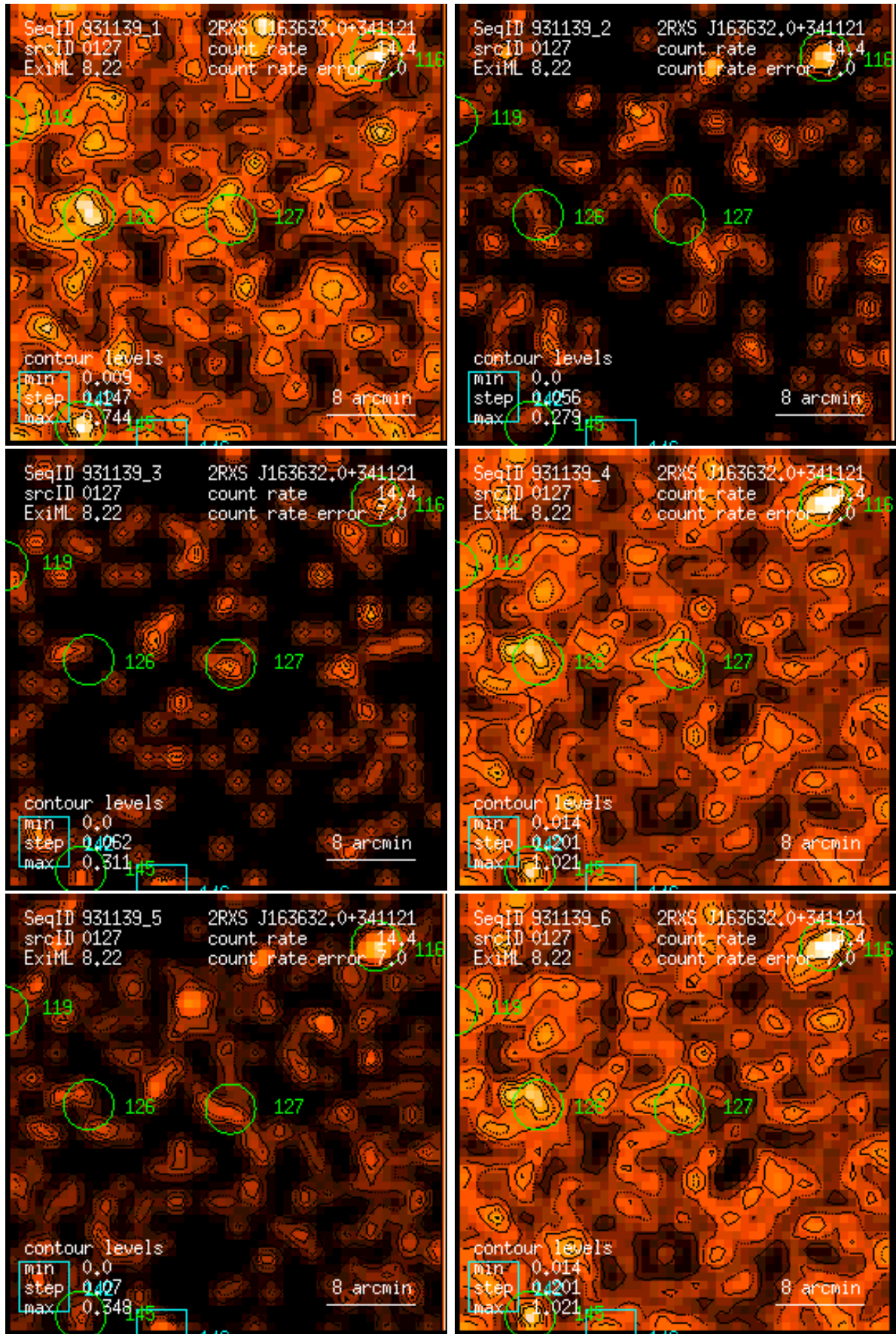
Figure 127: RASS 931139: detection 0127: band rate images, Gaussian filter: (1) PSPC channels 11 – 41, (2) 52 – 90, (3) 91 – 201, (4) 11 – 235, (5) 52 – 201, (6) 11 – 201. Broad band rates in counts/ks. Band rate contour levels in counts/ks/arcmin 2 .
