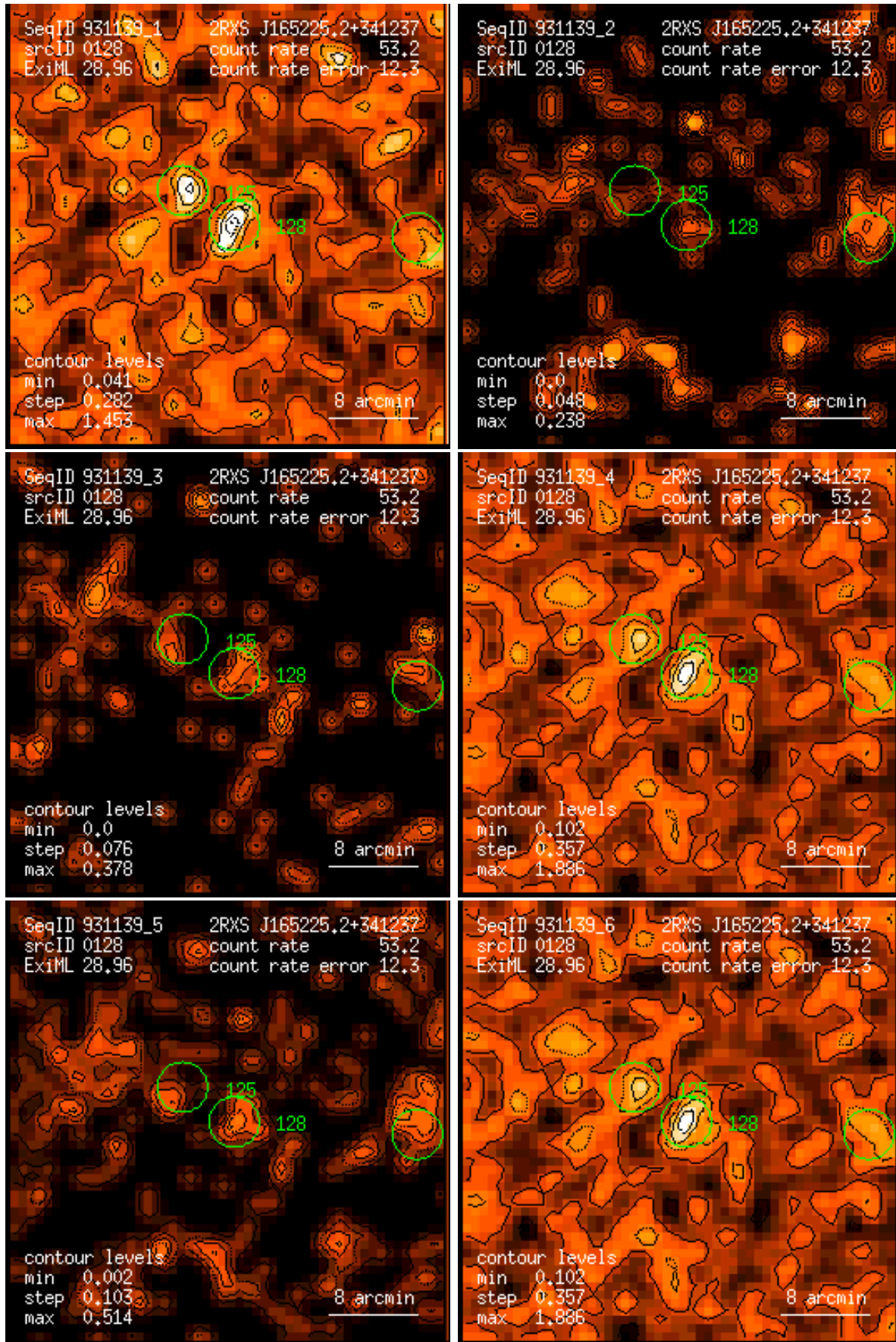
Figure 128: RASS 931139: detection 0128: band rate images, Gaussian filter: (1) PSPC channels 11 – 41, (2) 52 – 90, (3) 91 – 201, (4) 11 – 235, (5) 52 – 201, (6) 11 – 201. Broad band rates in counts/ks. Band rate contour levels in counts/ks/arcmin 2 .
