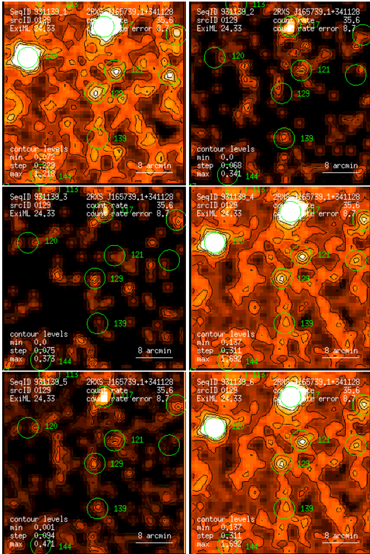
Figure 129: RASS 931139: detection 0129: band rate images, Gaussian filter: (1) PSPC channels 11 – 41, (2) 52 – 90, (3) 91 – 201, (4) 11 – 235, (5) 52 – 201, (6) 11 – 201. Broad band rates in counts/ks. Band rate contour levels in counts/ks/arcmin 2 .
